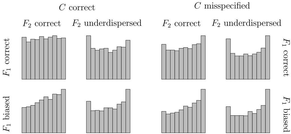
Figure 3: CopPIT histograms for the forecasters in the simulation study
