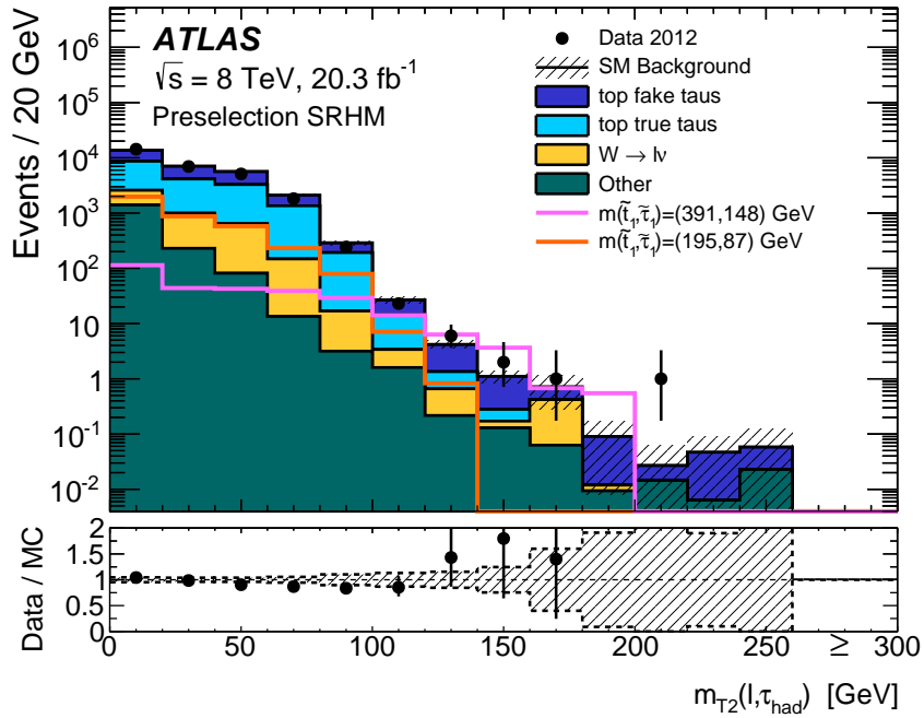
Figure 4: Top: distribution of the transverse mass constructed from the b -jet plus lepton and b -jet plus \tau_{\text{had}} , m_{T2}(b\ell, b\tau_{\text{had}}) , for events passing the lepton–hadron preselection requirements with the additional requirement of a second b -tagged jet. Bottom: distribution of the transverse mass constructed from the momenta of the light lepton and the hadronically decaying tau, m_{T2}(\ell, \tau_{\text{had}}) , for events passing the lepton–hadron preselection requirements. The contributions from all SM backgrounds are shown as a histogram stack; the bands represent the total uncertainty. The overflow bin in the m_{T2}(b\ell, b\tau_{\text{had}}) plot is filled with the events that have no (b\ell, b\tau_{\text{had}}) pairing satisfying m(b\ell) < m_t and m(b\tau_{\text{had}}) < m_t . The distributions expected for two signal models are also shown.
