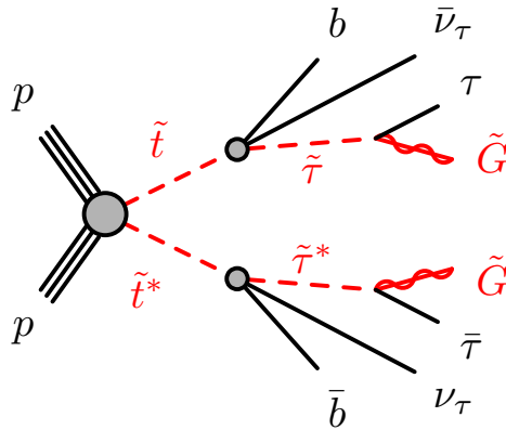
Figure 1: Diagram showing the decay topology of the signal process.
