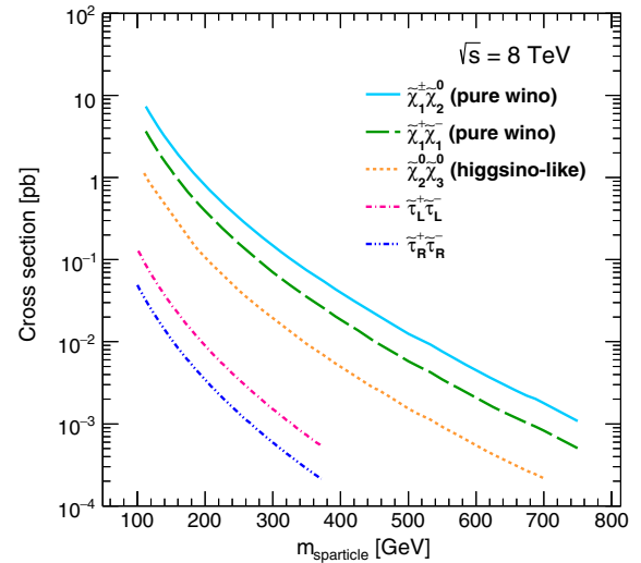
FIG. 1. The production cross sections for the simplified models of the direct production of \tilde{\chi}_1^\pm \tilde{\chi}_1^\pm , \tilde{\chi}_1^\pm \tilde{\chi}_2^0 [where m(\tilde{\chi}_1^\pm) = m(\tilde{\chi}_2^0) ], \tilde{\chi}_2^+ \tilde{\chi}_3^0 [where m(\tilde{\chi}_2^+) = m(\tilde{\chi}_3^0) ], and \tilde{\tau}^+ \tilde{\tau}^- studied in this article. The left-handed and right-handed stau-pair production cross sections are shown separately.
