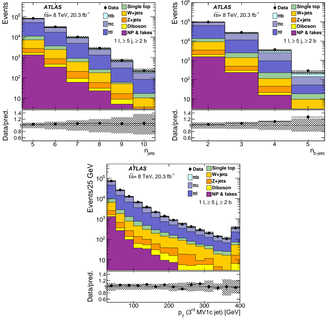
Figure 1: Jet multiplicity, b -tagged jet multiplicity, and transverse momentum p_T of the jet with the third highest MV1c value in the lepton-plus-jets channel. Events are required to have at least five jets, at least two b -tagged jets and one lepton. The data are shown as black points with their statistical uncertainty. The stacked distributions are the nominal predictions from Monte Carlo simulation; the hashed area shows the total uncertainty on the prediction. The bottom sub-plot shows the ratio of the data to the prediction. The non-prompt and fake lepton backgrounds are referred to as ‘NP & fakes’. The last bin of the distribution includes the overflow.
