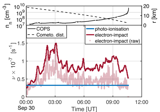
Figure 6. Top: Time series of the COPS neutral number density (full line) and cometocentric distance (dashed line). Bottom: Time series of the effective photoionization frequency \nu_{3.8\text{ au}}^{hv} (blue curve), electron-impact ionization frequencies corrected with the spacecraft potential (red curve) and uncorrected (pink dots). Pure water has been assumed for the neutral composition.
