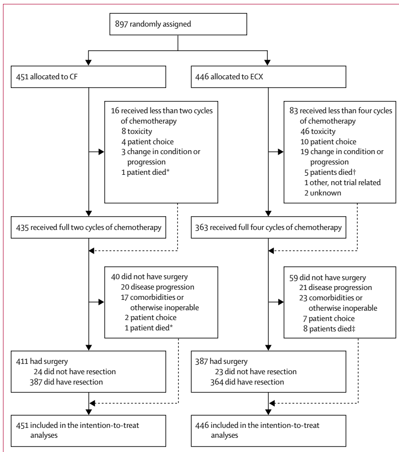
Figure 1: Consort diagram
