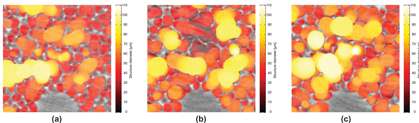
Fig 9. Structure diameters. Structure diameters obtained by air volume thickness map calculation with the 1.1 \mu\text{m} -pixel-size optics for three different peak inspiratory pressures: (a) 5 \text{cmH}_2\text{O} ; (b) 10 \text{cmH}_2\text{O} ; (c) 25 \text{cmH}_2\text{O} .
