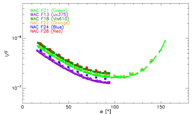
Figure 3. Multiwavelength coverage in MTP020 phase-function series. The reflectivity in all used filters is plotted against the phase angle.
