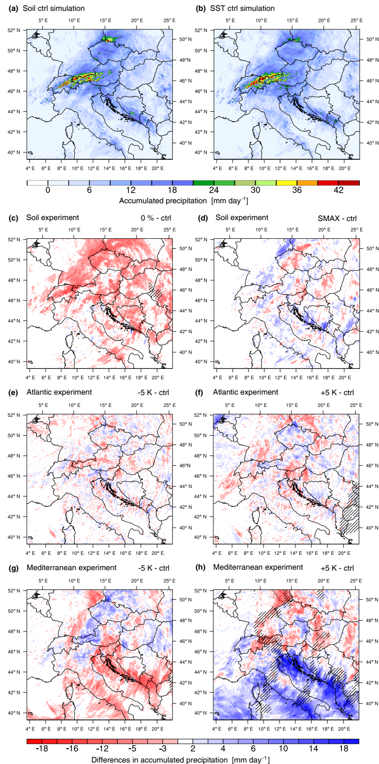
Figure 5. Panel (a) shows the accumulated precipitation (mm day -1 ) for the control simulation of the soil moisture experiments averaged over the five Vb events. Panel (b) shows the same as panel (a) but for the SST experiments. The second to fourth rows show the differences between the mean daily precipitation obtained by the different sensitivity experiments and the control simulation (mm day -1 ). Panel (c) shows the complete drainage soil experiment, panel (d) the full saturation soil experiment, panels (e) and (f) the –5 and +5 K Atlantic SST experiments, respectively, and panels (g) and (h) the –5 and +5 K Mediterranean SST experiments. The hatched area denotes significant changes at the 5 % significance level using a non-parametric Mann–Whitney U test.
