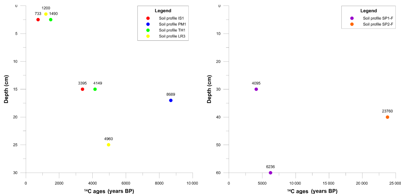
Figure 2. n -Alkane 14 C ages for soil profiles from the Black Rock Desert, Utah, USA (left), and Fuerteventura, Canary Islands, Spain (right). All 14 C ages are plotted as calibrated ages. IS1 is Ice Springs 1, PM1 is Pot Mountain 1, TH1 is Tabernacle Hill 1, LR3 is Lava Ridge 3, SP1-F is stone pavement sample location 1 – Fuerteventura and SP2-F is stone pavement sample location 2 – Fuerteventura.
