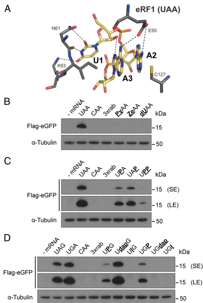
Fig. 4. Eukaryotic termination at modified stop codons. (A) Potential hydrogen-bond interactions (dashed lines) between eRF1 (dark gray) and the UAA stop codon (yellow) in a U-turn-like conformation (37). (B–D) Modified stop codons were incorporated in Flag-eGFP reporter mRNAs and were transfected into HEK293T cells. Twenty-four hours after transfection, the Flag-tagged translation products were detected by Western blotting. LE, long exposure; SE, short exposure.
