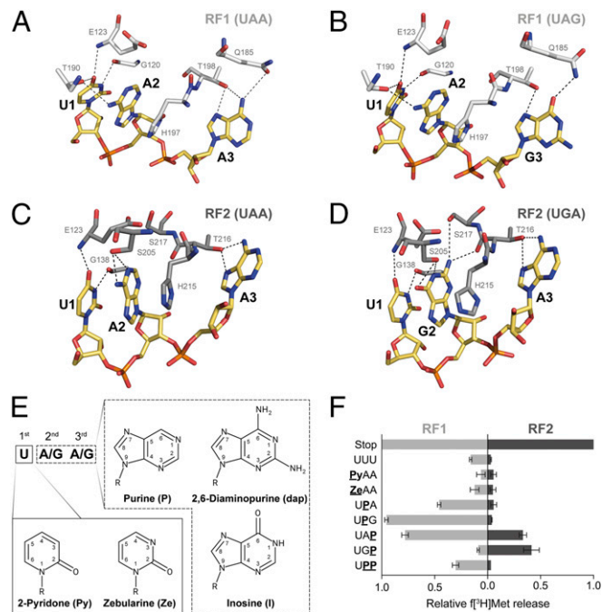
Fig. 1. (A–D) Interactions between residues of bacterial RFs and the three stop codons at the decoding site. RF1 (white) and RF2 (gray) sense the stop codons (yellow) UAA (A) and UAG (B) or UAA (C) and UGA (D), respectively, by forming a set of hydrogen bonds (dashed lines; Escherichia coli numbering is used for RF residues; modified from refs. 32–35). (E) These interactions were modulated by the use of modified RNA bases within the stop codons. (F) The ability of RFs to recognize modified stop codons was determined by using a peptide release assay (error bars indicated SDs from the mean of three independent experiments).
