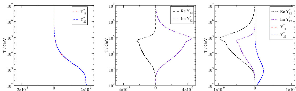
Figure 2. Averaged values of the density matrices, Y_{IJ}^{\pm} \equiv \frac{1}{s} \int_{\mathbf{k}_T} \tilde{\rho}_{IJ}^{\pm} , as a function of T/\text{GeV} . Left: the helicity-symmetric diagonal components. Middle: the helicity-antisymmetric non-diagonal components. Right: the remaining components, which are of similar magnitude as the baryon asymmetry.
