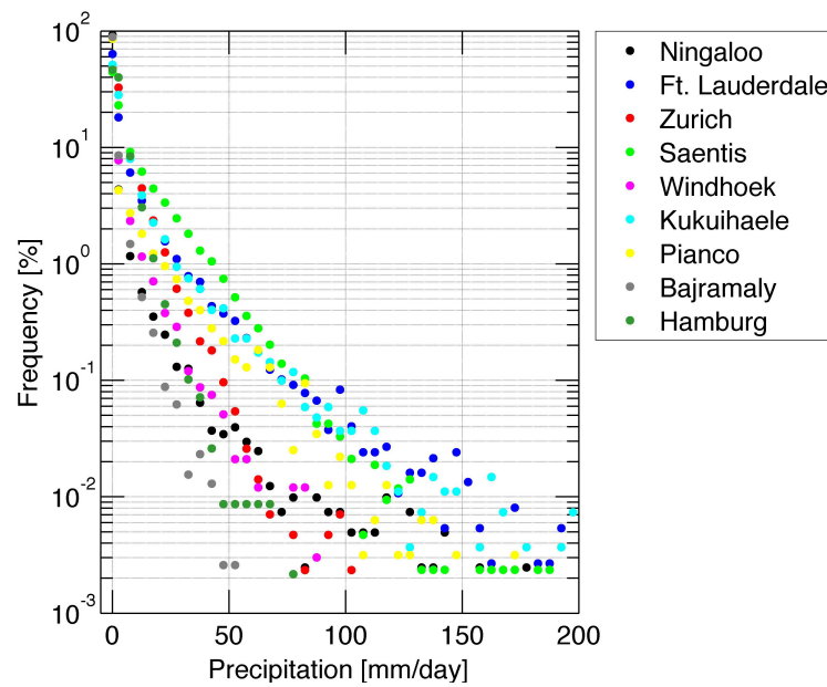
Figure 3. Frequency of precipitation as a function of the intensity of precipitation for the nine selected stations.
