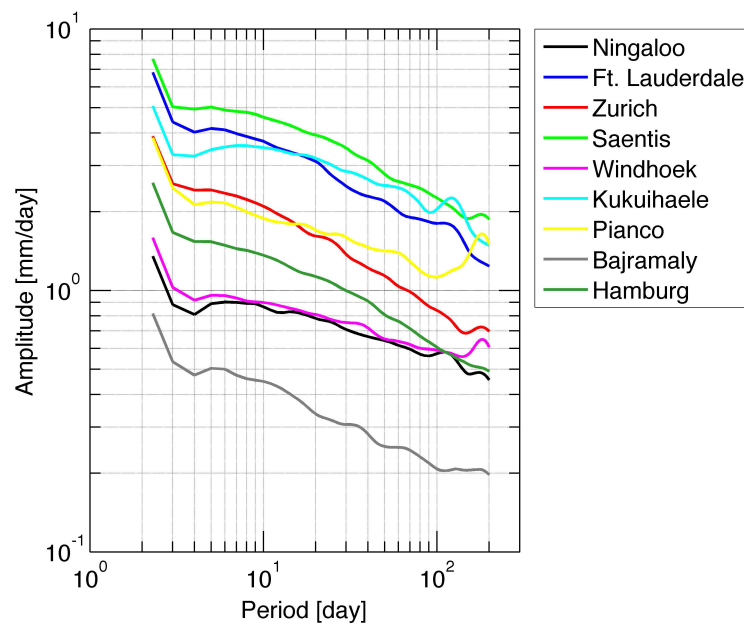
Figure 4. Amplitude spectra of precipitation for the period range from 2.3–200 days. The amplitudes were determined by a wavelet-like analysis.
