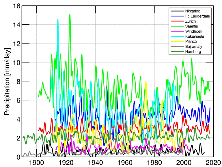
Figure 2. Interannual variability of precipitation at the nine selected stations. The curves were obtained by filtering the precipitation series with a 1.5-year low pass filter.
