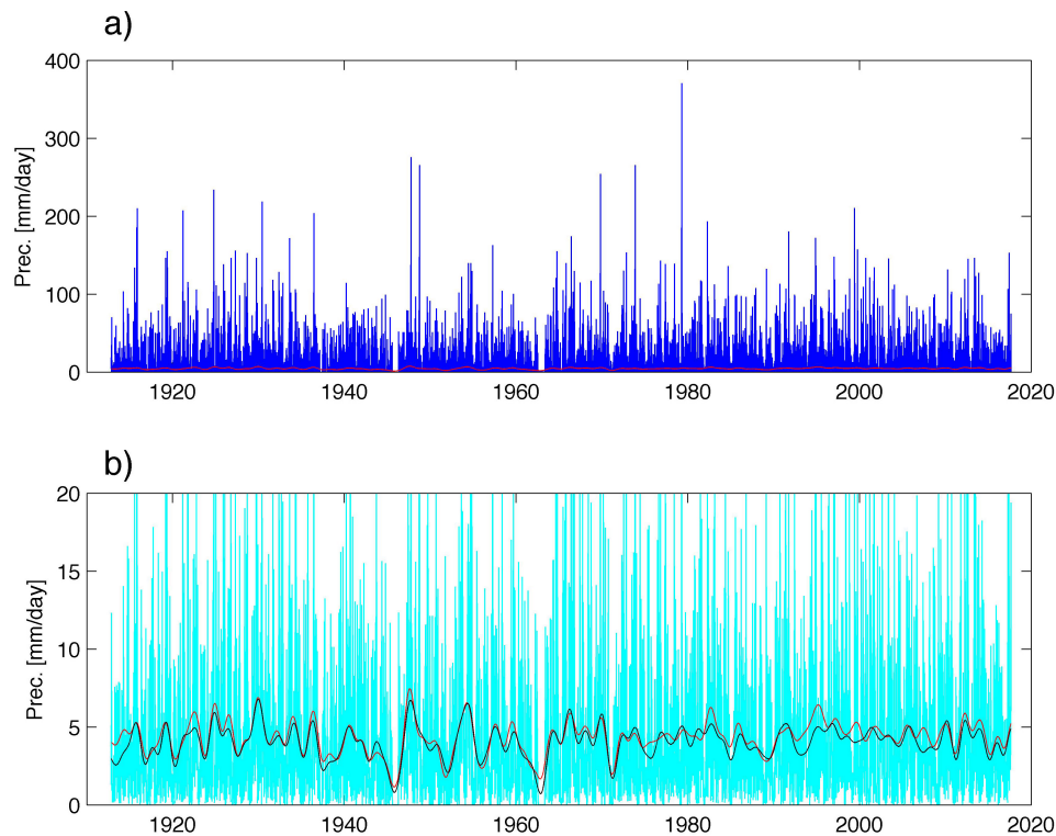
Figure 1. (a) Time series of precipitation at Ft. Lauderdale (blue line) and its interannual variability (red line), which was obtained by a 1.5-year low pass filter. (b) Time series of the amplitude of four-day fluctuation of precipitation at Ft. Lauderdale provided by a four-day band pass filter (cyan line). The black line denotes the 1.5-year low pass filtered data of the four-day amplitude series. For intercomparison, the interannual variability of (a) is also shown in (b) as a red line.
