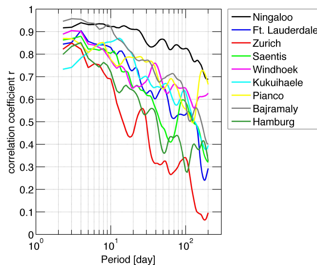
Figure 5. Correlation between the interannual variation of precipitation and the amplitude series obtained by band pass filtering at periods in the range from 2.3 days–200 days. Before calculation of the correlation coefficient, the amplitude series were filtered by a 1.5-year low pass filter.
