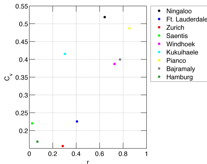
Figure 8. Coefficient of variation C_v of annual precipitation as a function of the correlation r between the amplitude of the annual oscillation and the interannual variability.
