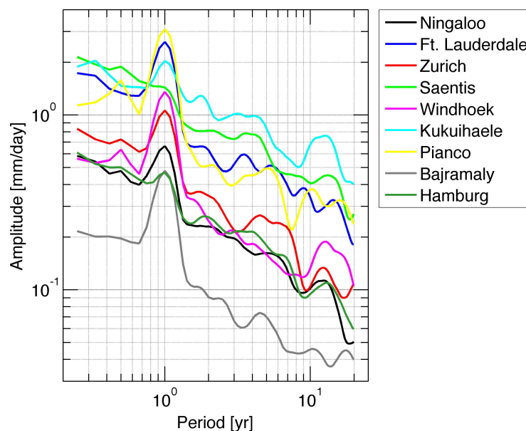
Figure 6. Amplitude spectra of precipitation for the period range from 3 months–20 years. The amplitudes were determined by a wavelet-like analysis.
