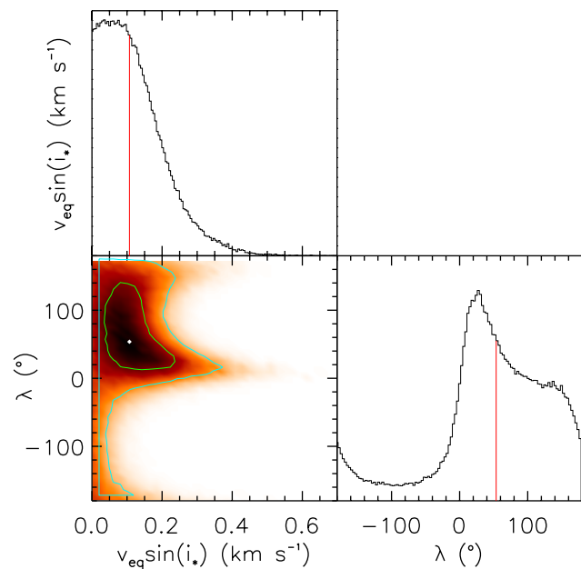
Fig. 5. Correlation diagrams for the posterior probability distributions of the solid-body stellar rotation model parameters. Green lines show the 1 and 2 \sigma simultaneous 2D confidence regions that contain 39.3% and 86.5%, respectively, of the accepted steps. 1D histograms correspond to the distributions projected on the space of each parameter. The red lines and white point show median values.
