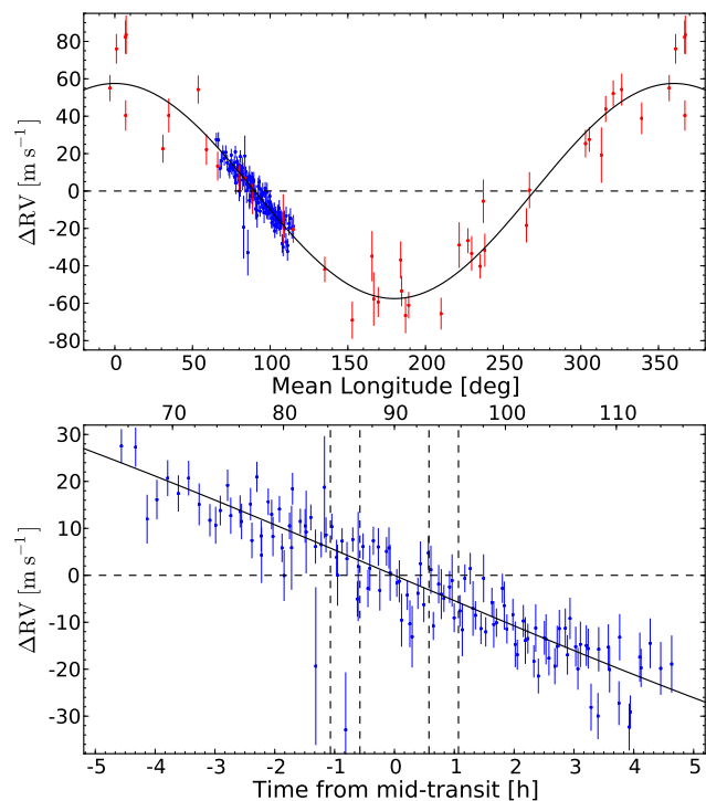
Fig. 2. Upper panel: Radial velocity measurements of WASP-49 with CORALIE (red points) and HARPS (blue points). The measures are fitted with a Keplerian orbit onto the DACE platform (see Sect. 2.4). The result is compatible with the circular orbit shown here. Lower panel: Zoom in on the three HARPS sequences only. The transit timing is indicated with dashed vertical lines representing the four contact points. No obvious Rossiter-McLaughlin effect is noticeable.
