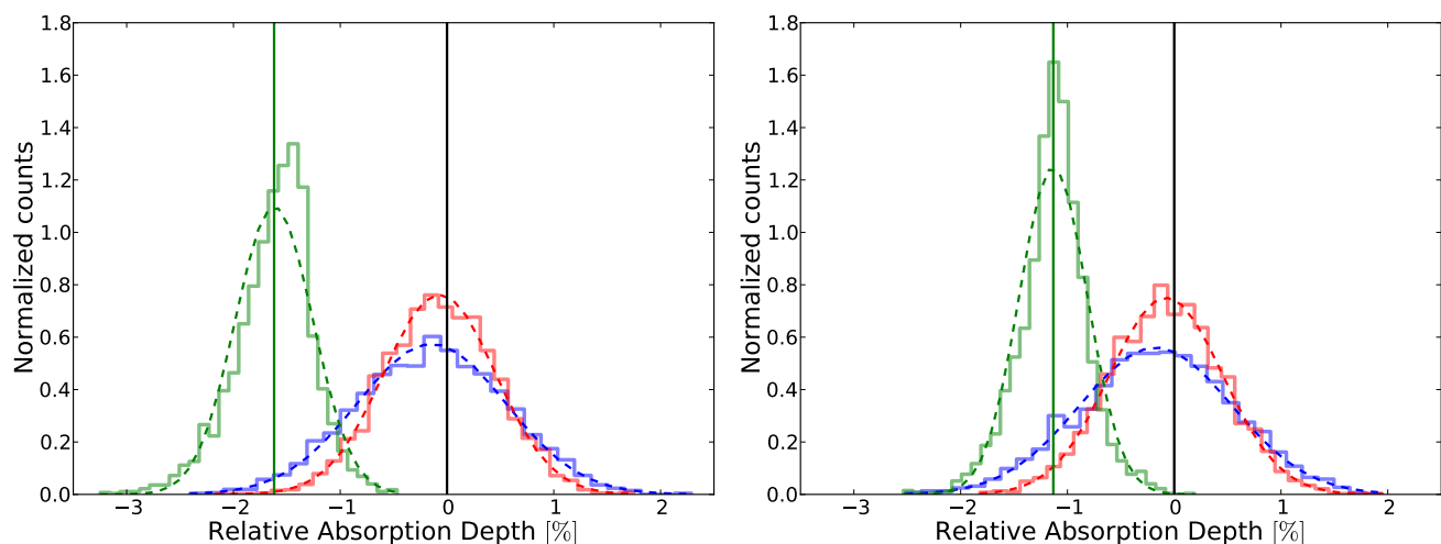
Fig. 9. Distribution obtained with the empirical Monte Carlo analysis for the Na I D 2 line (left) and D 1 line (right). In-in, out-out, and in-out distribution (continuous lines) are shown in blue, red, and green with their respective Gaussian fit (dotted lines). The green vertical lines are the averages values of the in-out distribution.
