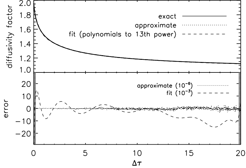
Figure A1. Calculations of the diffusivity factor using a canned routine (“exact”) versus those performed using our fitting formulae for \mathcal{E}_1 in equation (A1) (“approximate”). The calculation labeled “fit” is a 13th order polynomial fit to the exact solution, which performs poorly even at the \sim 10^{-3} level.
