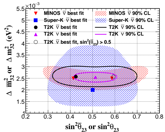
FIG. 2. 90% confidence regions for \sin^2(\theta_{23}) and \Delta\bar{m}_{32}^2 in \nu mode (corresponding to 7.482 \times 10^{20} POT) and \bar{\nu} -mode (corresponding to 7.471 \times 10^{20} POT). Normal hierarchy is assumed. 90% confidence regions obtained by SK [41] and MINOS [42] for \bar{\nu} are also shown. The best fit in the case \sin^2(\theta_{23}) > 0.5 is also displayed for comparison with the MINOS result.
