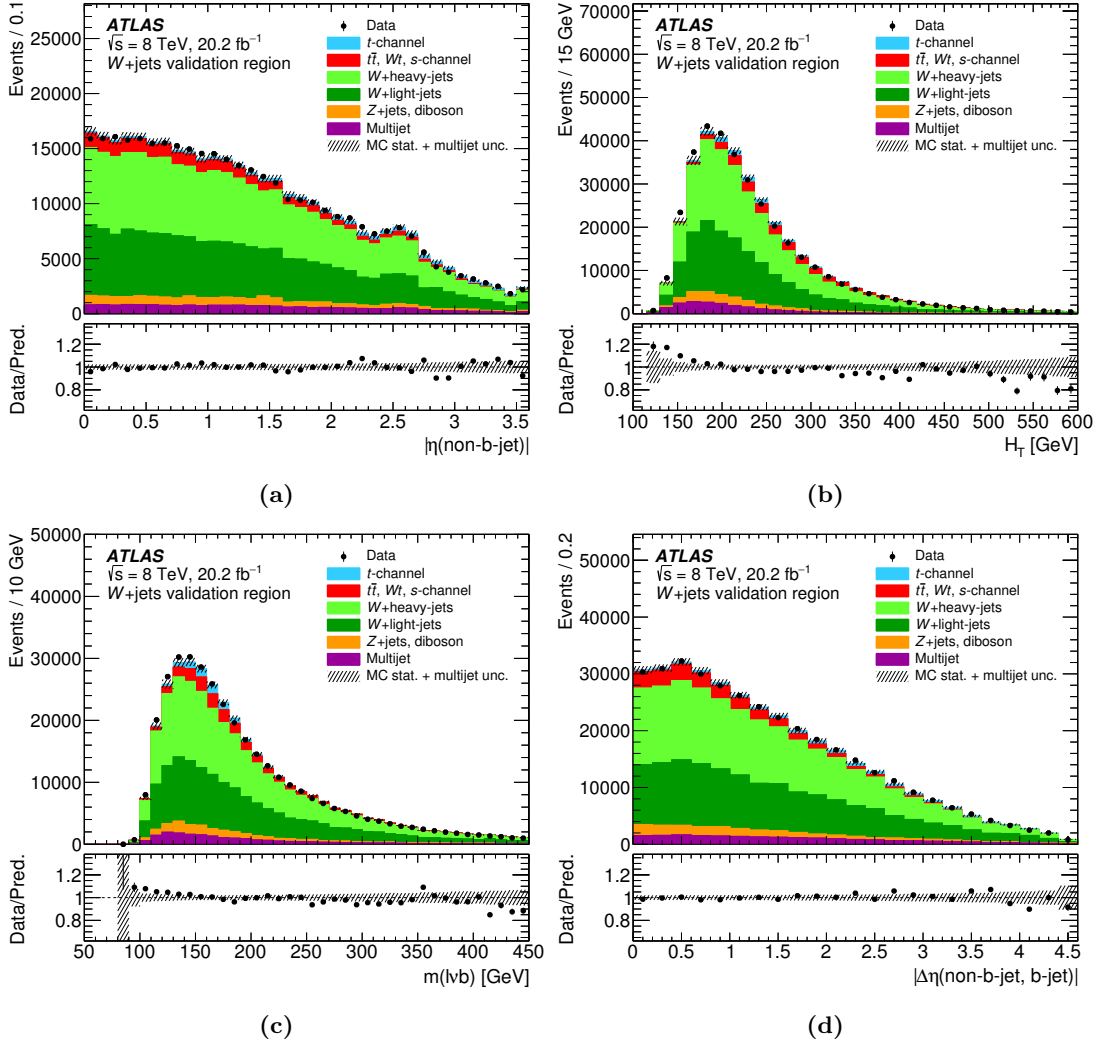
Figure 6. Distributions of (a) |\eta(\text{non-}b\text{-jet})| , (b) the scalar sum of the p_T of all final-state objects, H_T , (c) reconstructed top-quark mass, m(\ell\nu b) , and (d) |\Delta\eta(\text{non-}b\text{-jet}, b\text{-jet})| in the W +jets validation region for the merged electron and muon channels. The multijet background is estimated using data-driven techniques, while contributions from simulated W +jets, top-quark backgrounds and t -channel event samples are normalised to the results of a maximum-likelihood fit to event yields in the signal and control regions. The uncertainty bands correspond to the uncertainties due to the size of the simulated event samples added in quadrature with the data-driven normalisation uncertainty of 70% estimated for the multijet contribution. The lower plots show the ratio of data to prediction in each bin.
