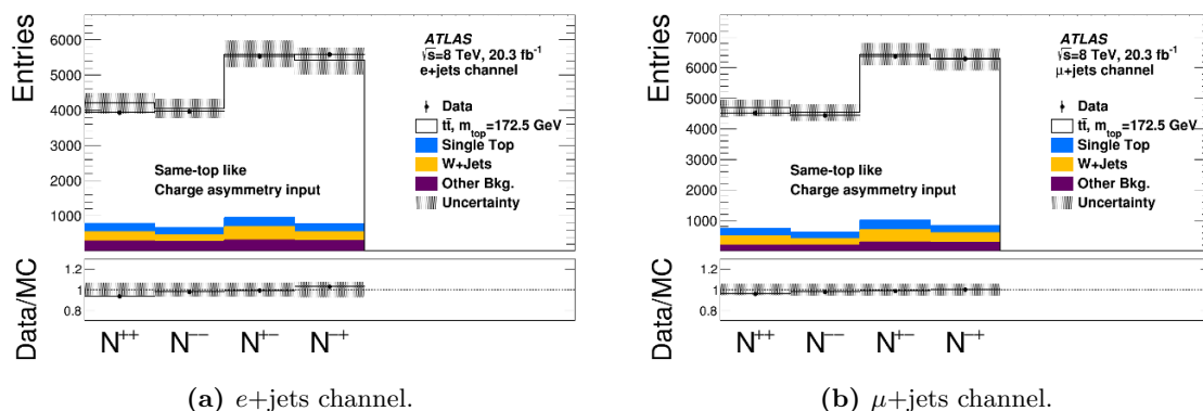
Figure 3. Same-top-like charge-pairings distributions. The hashed area represents all experimental systematic uncertainties as well as the b -hadron production and hadron-to-muon branching ratio uncertainties. The lower panel of the distributions show the ratio of the data divided by the simulation. (a) shows the e +jets channel while (b) shows the \mu +jets channel.
