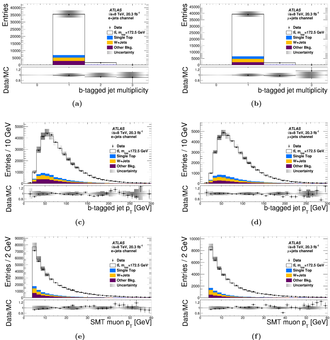
Figure 2. Distributions showing data and simulation. The hashed area represents all experimental systematic uncertainties as well as the b -hadron production and hadron-to-muon branching ratio uncertainties. The lower panel of the distributions show the ratio of the data divided by the simulation. The distributions on the left-hand side show the e +jets channel while the distributions on the right-hand side show the \mu +jets channel. (a) and (b) show the b -tagged jet multiplicity, (c) and (d) show the b -tagged jet p_T and finally (e) and (f) show the SMT muon p_T .
