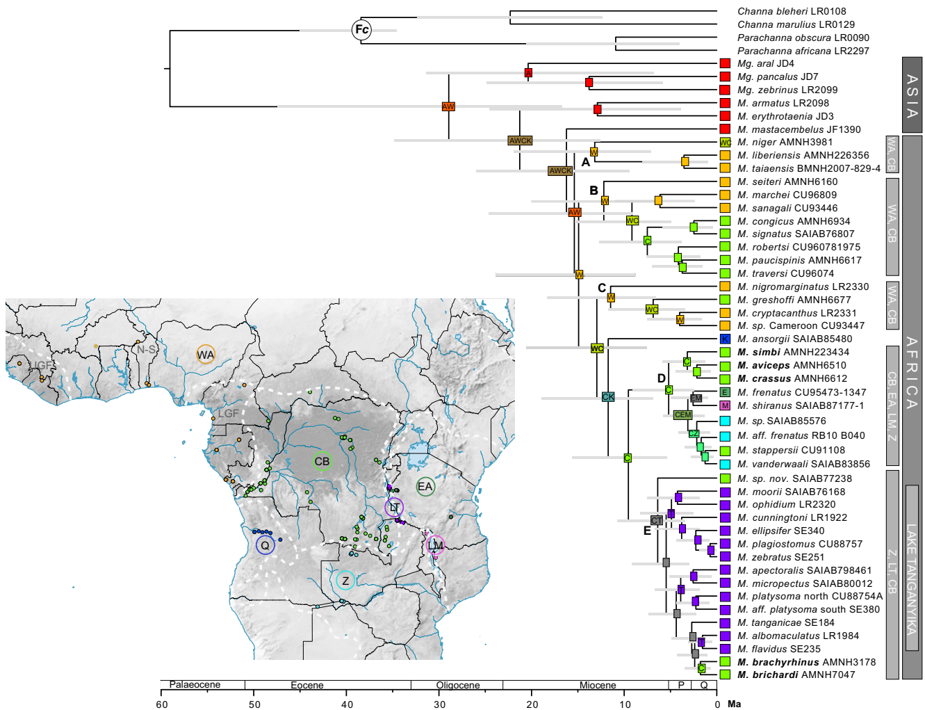
FIGURE 1 Spatiotemporal reconstruction of African Mastacembelus spiny eels. Dated nuclear tree inferred using a Bayesian relaxed clock (BEAST) including 95% confidence intervals (HPD). Biogeographic range inheritance based on the DEC model (M0) implementing BioGeoBEARS. Colours at species tips reflect geographic designations (see inset map for African regions [ichthyo-provinces] and Appendix S2); Asia (A, red); West Africa (W, light orange, including N-S, LGF, UGF regions); Congo Basin (C, light green), Zambezi (Z, aqua), Quanza (Q, dark blue), East Africa (E, dark green), Lake Tanganyika (T, purple), Lake Malawi (M, pink); C+W (olive). States at nodes represent the most probable ancestral area before an instantaneous speciation event; stem labels (state of the descendant lineages immediately after speciation) are omitted on this figure to help with clarity, but see these reconstructions in Appendix S3. AR, African radiation; A–E, main clades; Fc, fossil calibration node; Lower Congo River endemics in bold [Colour figure can be viewed at wileyonlinelibrary.com ]
