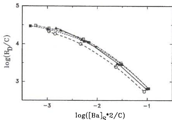
Fig. 1. Sorption data for barium in synthetic groundwater on <32- \mu m glaciofluvial material subjected to various chemical treatments; for clarity desorption data are omitted; distribution ratios normalized with the cation exchange capacity C .
