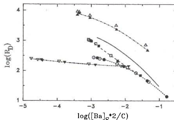
Fig. 2. Sorption ( \nabla, \bullet, \blacksquare, \blacktriangle ) and desorption ( \nabla, \circ, \square, \triangle ) data for barium on clay minerals and on <32- \mu m glaciofluvial material in synthetic groundwater.
