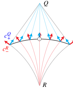
FIGURE 3. The two loops c_+^Q and c_-^R on the surface S_{2,q,r}^Q .
