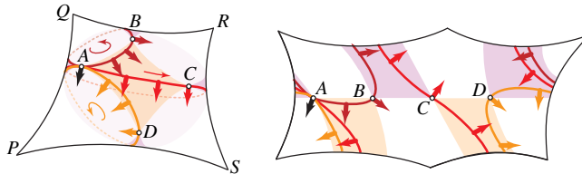
FIGURE 11. The curves c^{AB} , c^{AC} and c^{AD} on S_{p,q,r,s}^A . The black tangent vector is their common intersection point. The orientations are represented on the left by thinner arrows.
