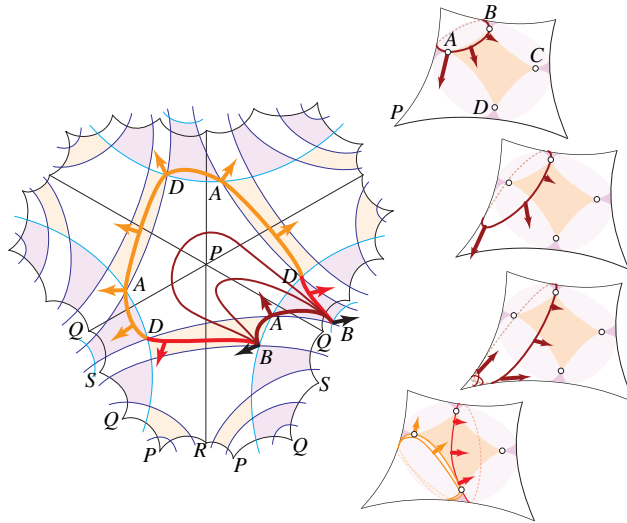
FIGURE 13. Transportation of the loop c^{AB} by the geodesic flow keeping the point that belongs to the fiber of B fixed. The image crosses the fiber of P (here we have p = 3 ). After some time, it reaches S_{p,q,r,s}^D and is then isotopic to c^{DB} + (p-1)c^{DA} .
