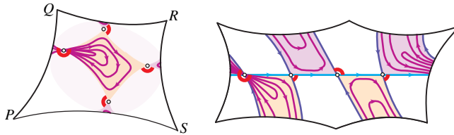
FIGURE 10. The foliation of T_1 \cup T_2 by the family (\alpha_s(t))_{s,t \in (0,1)} . The unit tangent vectors form the surface S_{p,q,r,s}^A .
