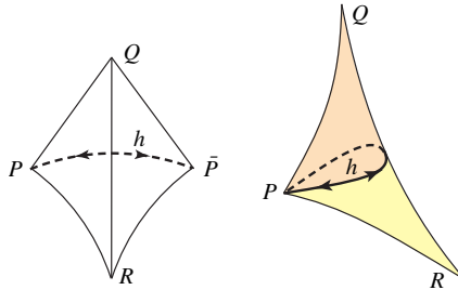
FIGURE 1. The orbifold \mathbb{H}^2/\Gamma_{2,q,r} (on the right) and a fundamental domain (on the left). The two Birkhoff sections S_{2,q,r}^Q and S_{2,q,r}^R consist of those tangent vectors based on the geodesic h and pointing to the Q -side (respectively the R -side) of h .
