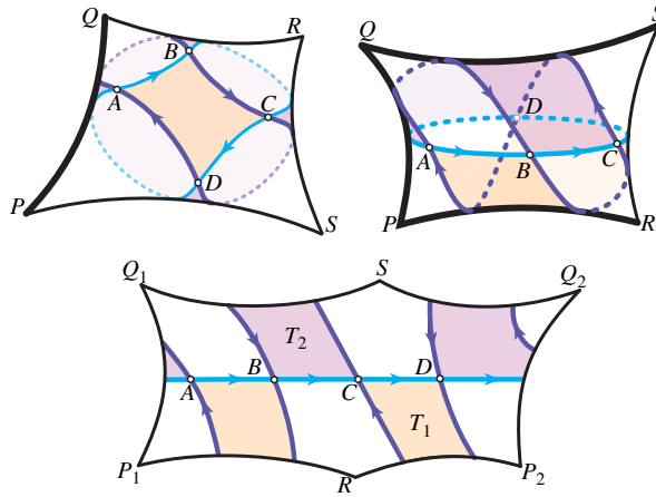
FIGURE 9. Two views of an orbifold with four singular points P, Q, R, S and a fundamental domain obtained by cutting along RP, PQ and QS . The two geodesics b_1 and b_2 are shown in bold. They intersect at four points, called A, B, C and D . The two quadrangles T_1, T_2 are colored.
