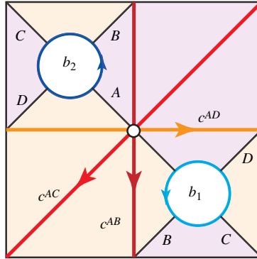
FIGURE 12. The torus S_{p,q,r,s}^A with its two boundary components b_1, b_2 and the curves c^{AB}, c^{AC} and c^{AD} . The fibers of the points A, B, C and D are also drawn.
