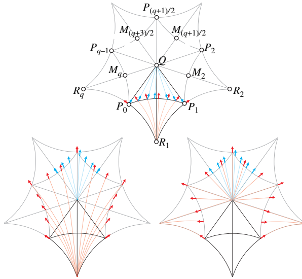
FIGURE 4. (a) The names of various points. (b) The images of the curves c_+^+ and c_-^- under the map \Phi^Q : S_{2,q,r}^Q \rightarrow S_{2,q,r}^R . (c) The curves \Phi^Q(c_+^+) and \Phi^Q(c_-^-) are homotoped onto c_-^- and (q-2)c_-^- - c_+^+ .
