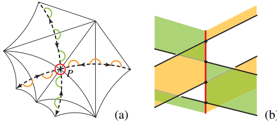
FIGURE 2. (a) The union of four fundamental domains for \mathbb{H}^2/\Gamma_{2,q,r} , and four copies of S_{2,q,r}^Q . (b) The surface S_{2,q,r}^Q in a neighborhood of P , before modding out by the lift of the order-two rotation around P . It is a topological surface. Since the lift of the order-two rotation in the unit tangent bundle is an order-two screw-motion with no fixed point, we still obtain a topological surface when modding out.
