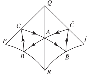
FIGURE 5. The geodesic b on \mathbb{H}^2/\Gamma_{p,q,r} travels along the two orthic triangles of PQR and \bar{P}QR .
