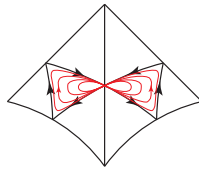
FIGURE 6. The foliation (\alpha_s) of the interior of b by butterfly-like curves.
