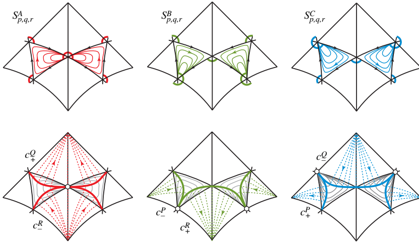
FIGURE 7. The three surfaces S^A_{p,q,r} , S^B_{p,q,r} and S^C_{p,q,r} (top) and some loops on each of them (bottom).
