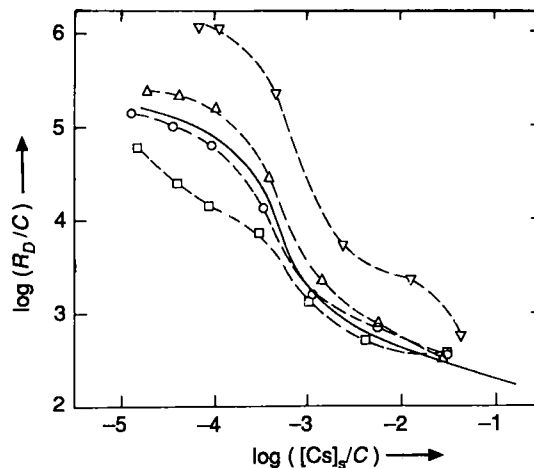
Fig. 6. Sorption of cesium in synthetic groundwaters of different composition (size fraction: <32\text{ }\mu\text{m} from Glattfelden, depth: 22–24m). — SGW; ○ SGW-1/2[Ca, Mg]; △ SGW-1/3 K; ▽ SGW-0K; □ SGW-HCO 3 (see text).
