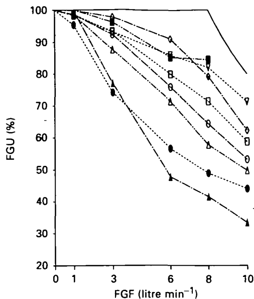
FIG. 2. Fresh gas utilization (FGU) for the anaesthesia breathing systems as a function of fresh gas flow (FGF). \square = Dräger Cicero; \circ = Dräger 8 ISO; \triangle = Dräger AV1; \nabla = Ohmeda Modulus II Plus; \diamond = Gambro Engström Elsa; \blacksquare = Siemens Servo Ventilator; \bullet = Siemens Ventilator 710; \blacktriangle = Megamed 700A; — = ideal.
