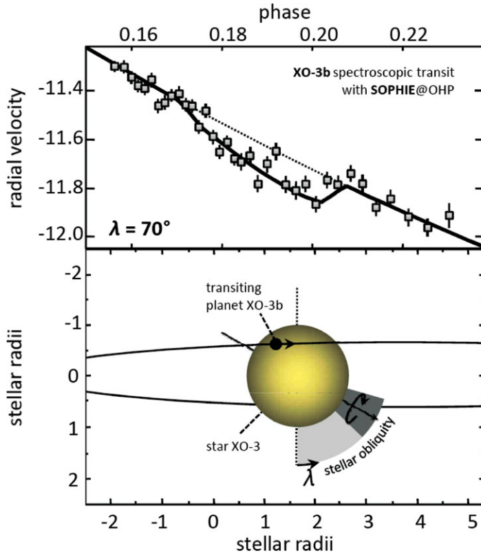
Figure 1. Top: Rossiter-McLaughlin effect models with \lambda = 70^\circ . The squares are the SOPHIE radial-velocity measurements of XO-3 with 1\text{-}\sigma error bars as a function of the orbital phase. The solid and dotted lines are the Keplerian fits with and without Rossiter-McLaughlin effect. Bottom: Schematic view of the XO-3 system with nearly transverse transit, as seen from the Earth. The stellar spin axis is shown, as well as the planet orbit and the \lambda misalignment angle (or stellar obliquity). The range \lambda = 70^\circ \pm 15^\circ which is favored by our observations is shown.
