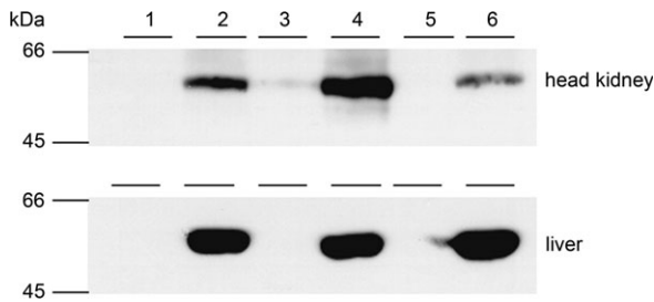
FIG. 3. Immunoblotting of CYP1A protein in head kidney and liver tissue of rainbow trout. The bands show CYP1A-immunoreactive protein of head kidney and liver microsomes from rainbow trout treated with BaP (25 mg/kg body weight, lanes 2, 4, 6) or corn oil (lanes 1, 3, 5) and sampled at 3 (lanes 1, 2), 6 (lanes 3, 4), and 10 (lanes 5, 6) days p.i., respectively. One hundred and thirty-six micrograms microsomal protein of head kidney and 24 \mu g microsomal protein of liver were added to each well, electrophoresed and blotted as described in "Material and Methods." The antibody used was the mAb C10-7 against peptide 277–294 of rainbow trout CYP1A (Biosense).
