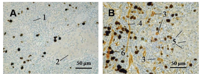
FIG. 5. Immunohistochemical localization of CYP1A by mAb C10-7 in head kidney of (A) control rainbow trout, and (B) rainbow trout treated with BaP (25 mg/kg body weight), 3 days p.i. (A) In control trout, no immunoreactivity is visible in lymphoid (1) and endocrine cells (2). (B) In BaP-treated fish, strong immunoreactivity is present in several cells of lymphoid cells (3), vascular endothelial cells (4), whereas no immunoreactivity is visible in endocrine cells (5). Pigmented cells (black spots) are also clearly visible (6).
