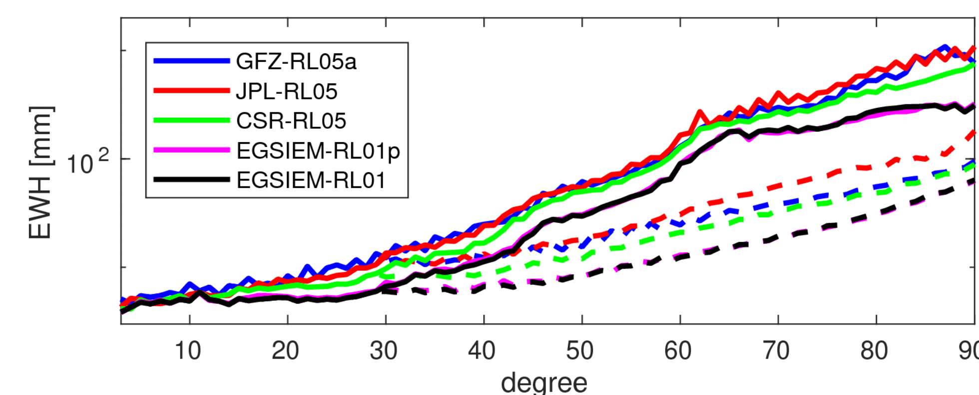
Fig. 5: Quality control in the spectral domain of the EGSIEM combination compared to the GRACE SDS time series. Shown is the RMS of degree amplitudes of anomalies, either including all orders (solid lines), or truncated at order 29 to focus on the signal dominated part of the spectrum (dashed).
