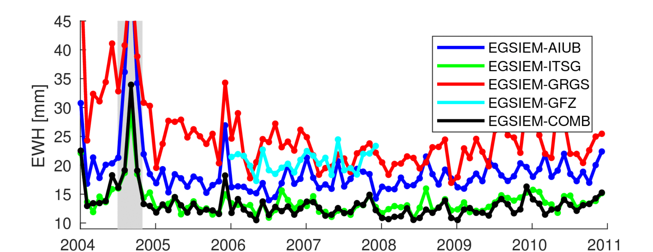
Fig. 8: Monthly RMS of EWH anomalies over the oceans for the extended time-series (smoothed by a 400km Gauss filter). Reduced quality during fall 2004 (gray box) coincides with a period of orbit resonance. The peak in RMS in 01/2004 is caused by reduced data quality, in 12/2005 a satellite swap manoeuvre took place. Note that during the availability of GFZ-EGSIEM the combination consists of four monthly contributions, otherwise only of three.
