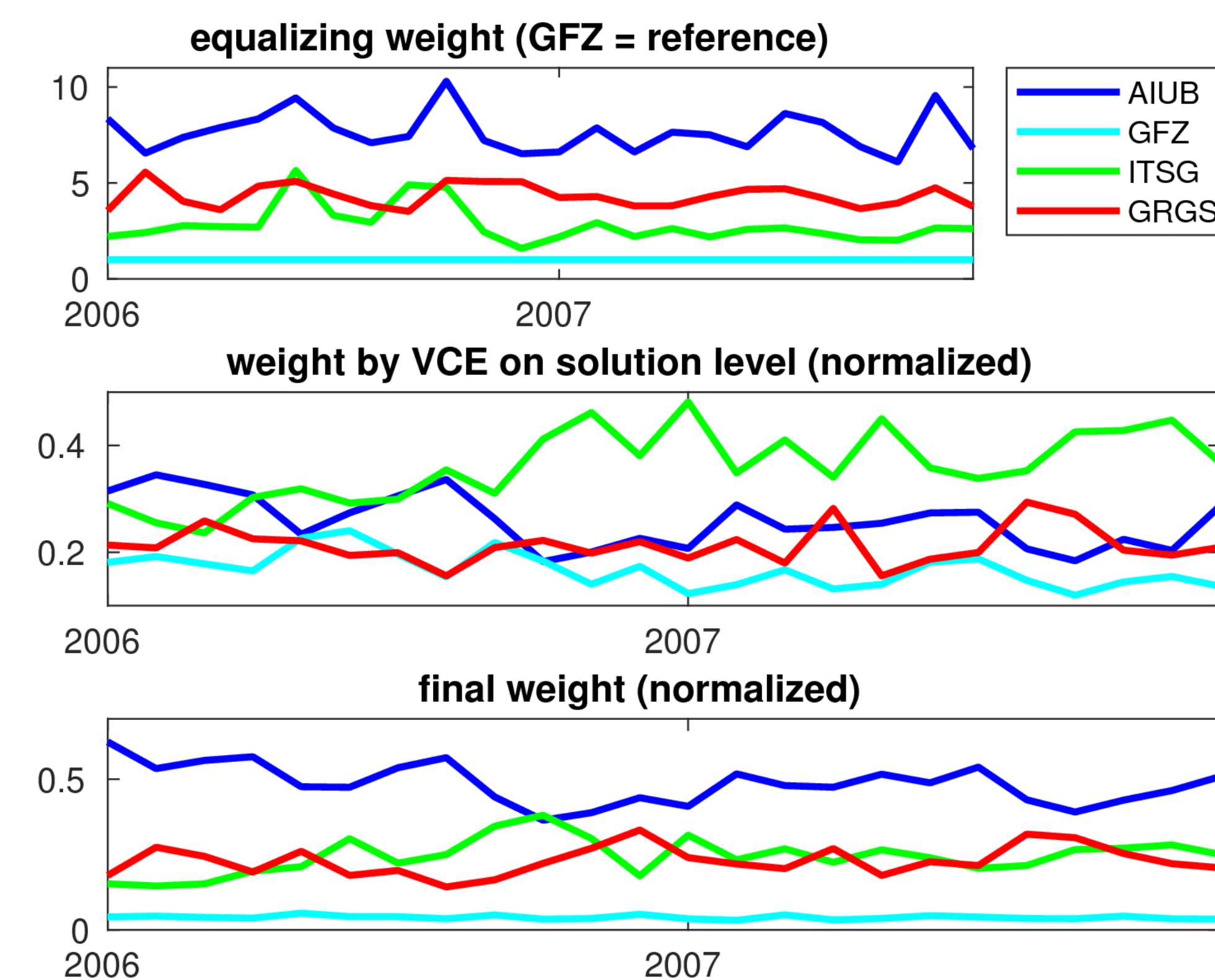
Fig. 3: Relative weights applied for the combination of the monthly NEQs: empirical scaling factors (top) account for the different parametrization, noise models and choice of observations (GPS phases versus kinematic orbits), weights derived by VCE on solution level (middle) represent the different noise levels of the individual contributions, the final weights (bottom) are the monthly products of the empirical factors and the relative weights based on the different noise levels.
