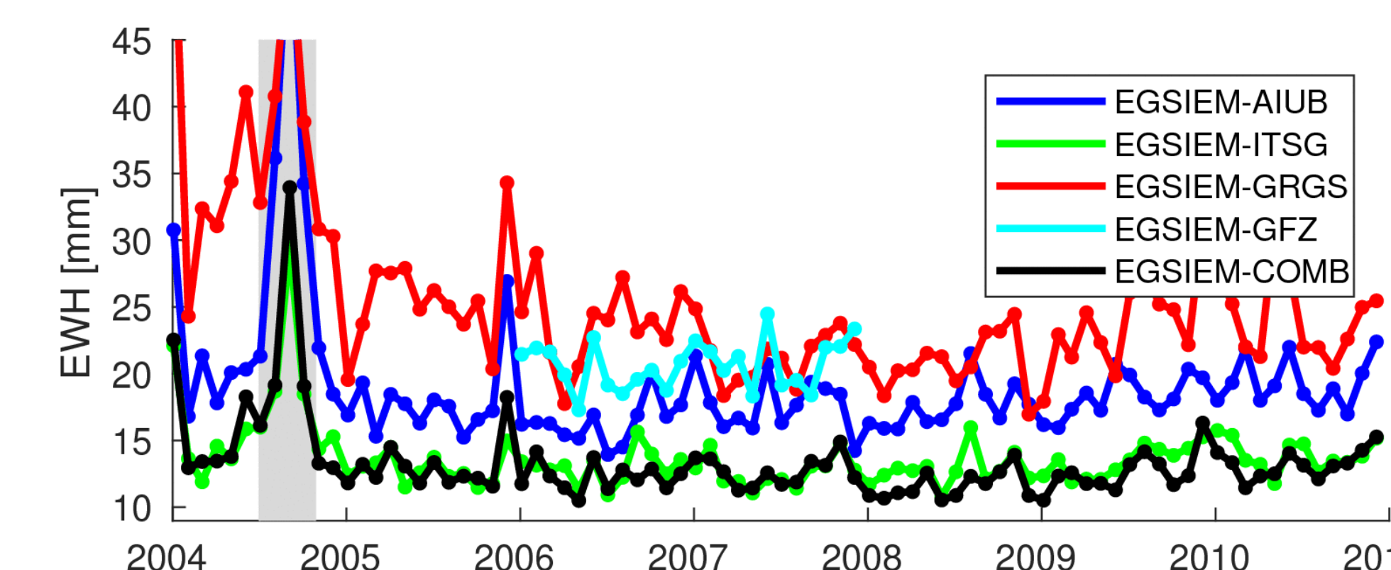
Fig. 8: Monthly RMS of EWH anomalies over the oceans for the extended time-series (smoothed by a 400km Gauss filter). Reduced quality during fall 2004 (gray box) coincides with a period of orbit resonance. The peak in RMS in 01/2004 is caused by reduced data quality, in 12/2005 a satellite swap manoeuvre took place. Note that during the availability of GFZ-EGSIEM the combination consists of four monthly contributions, otherwise only of three.
