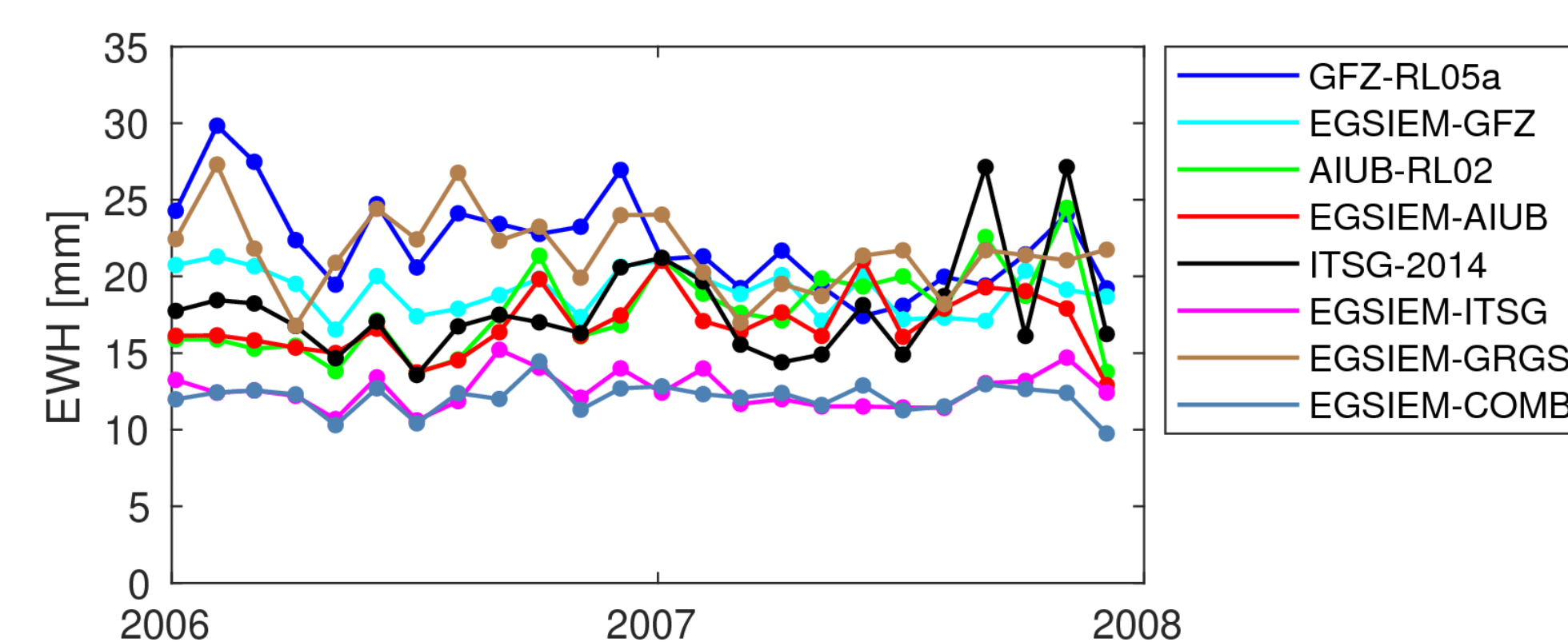
Fig. 4: Monthly quality control in the spatial domain of the ACs individual contributions, compared to the corresponding EGSIEM time-series and the combination. Shown is the RMS of anomalies over the oceans (smoothed by a 400km Gauss filter), weighted by the cosine of the latitude of the grid cells.
