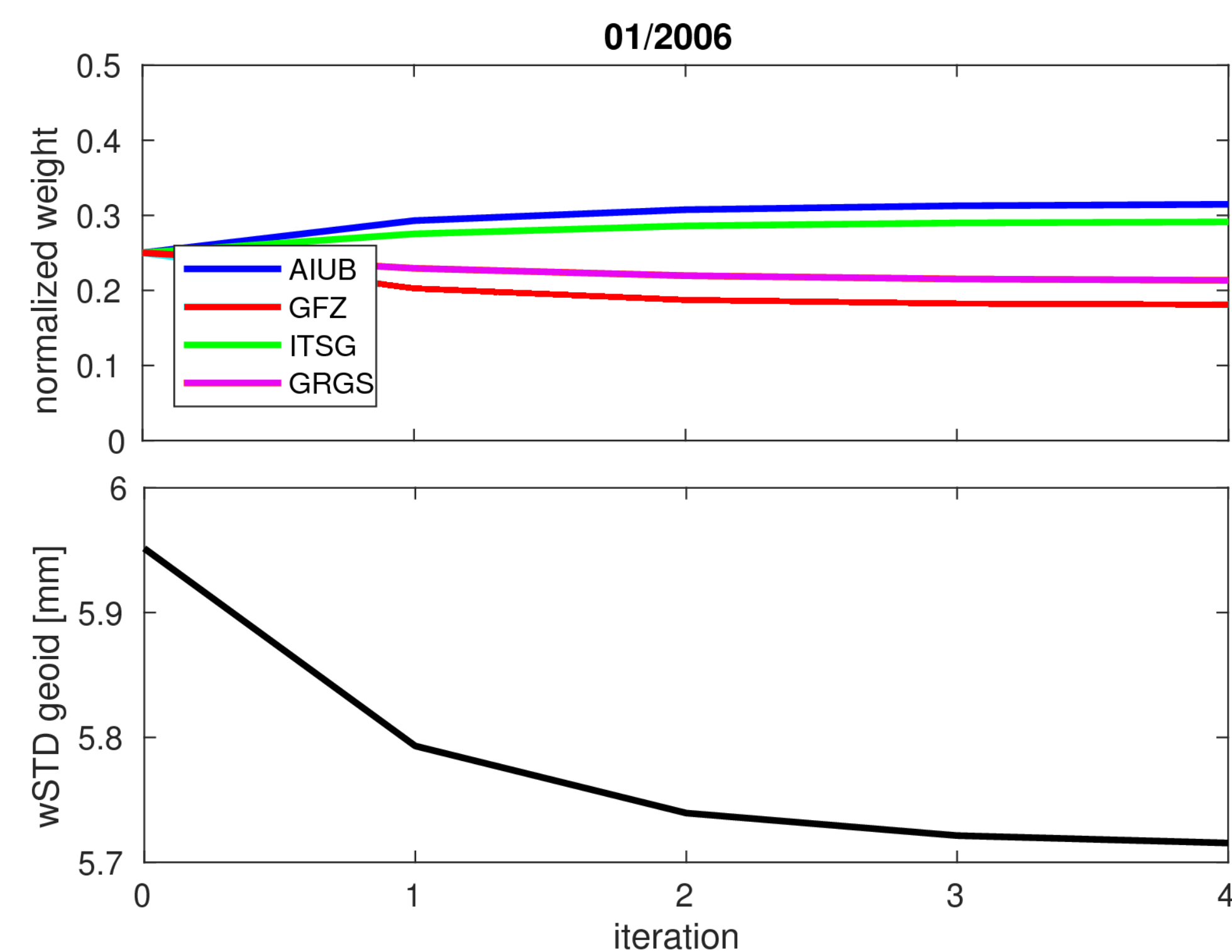
Fig. 2: Weights on solution level are derived iterative (top), the STD of anomalies over the oceans (bottom) indicates the corresponding noise.
