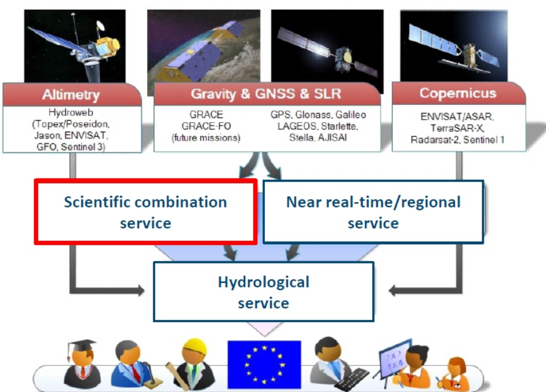
Fig. 1: EGSIEM has installed three services related to temporal gravity field variations.
