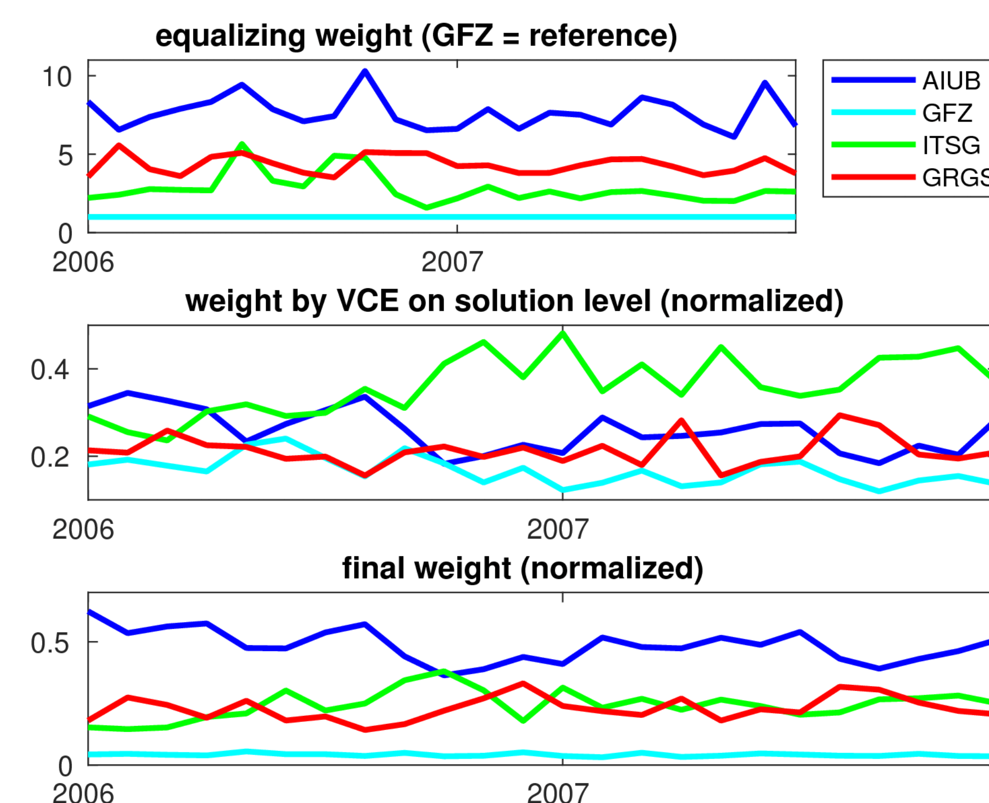
Fig. 3: Relative weights applied for the combination of the monthly NEQs:
