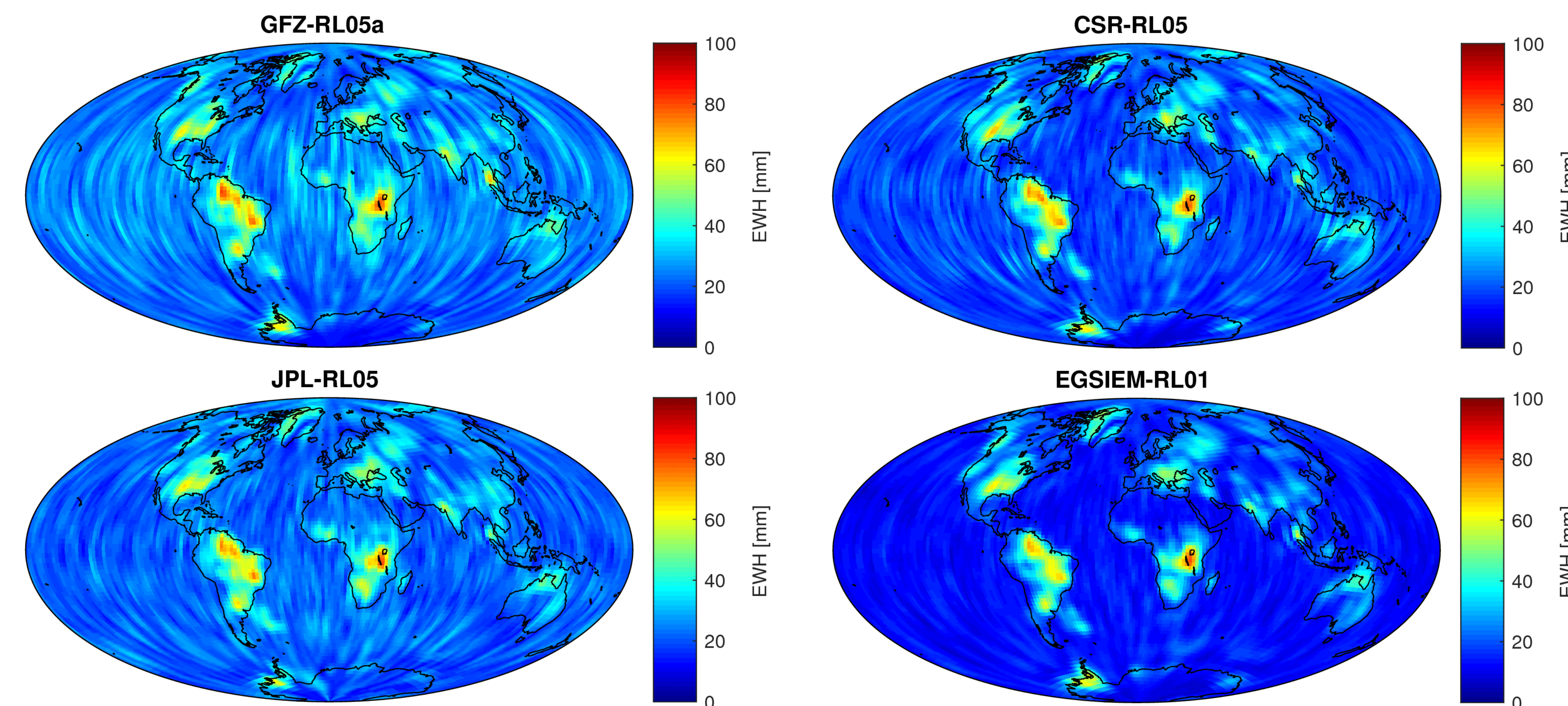
Fig. 6: For quality control the noise level of the combined EGSIEM gravity fields are compared to the official GRACE SDS time series. Shown are anomalies, i.e. residuals after removal of trends and seasonal variations. Over the oceans the anomalies mainly represent noise.
