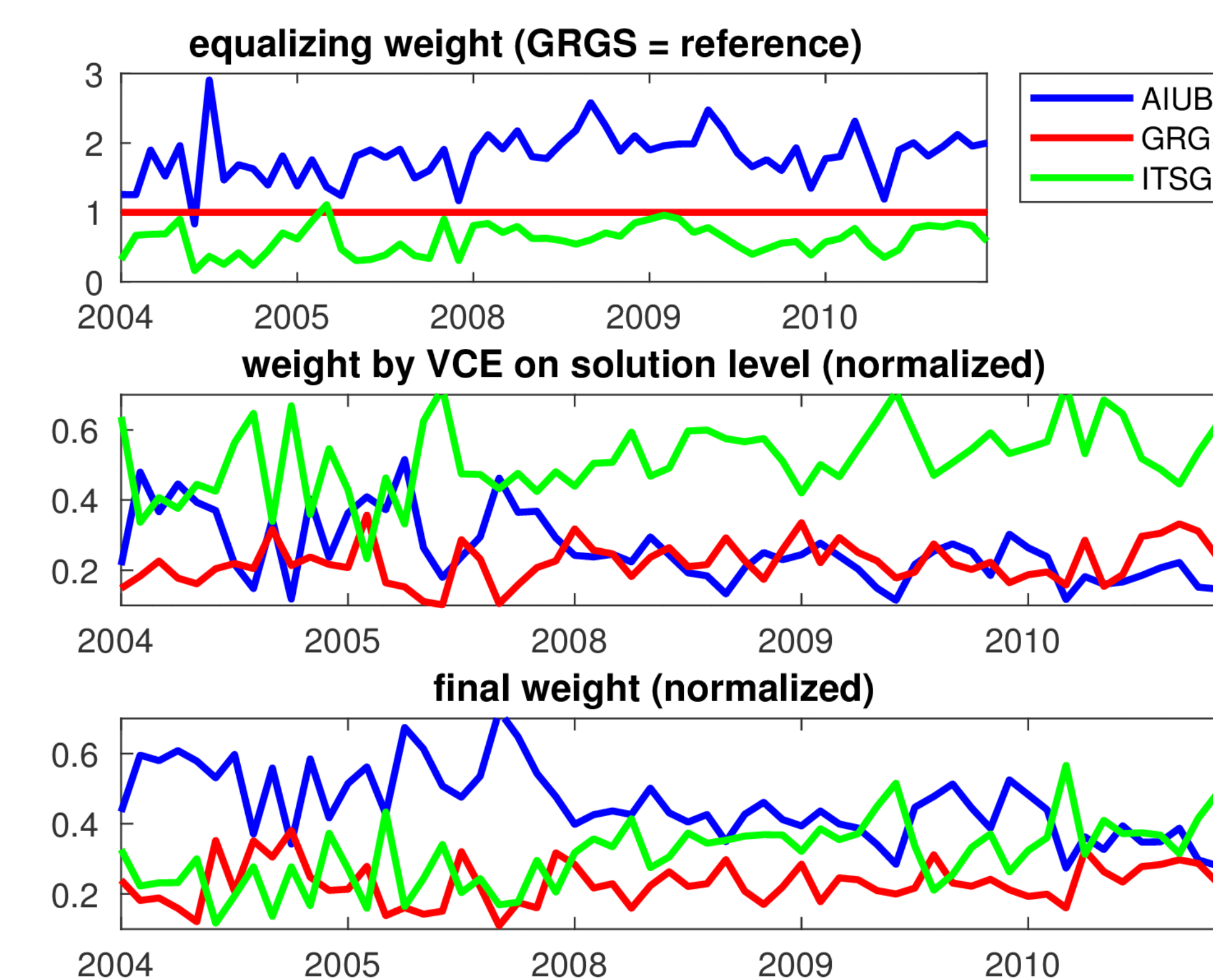
Fig. 7: Relative weights applied for the combination of the NEQs of the extended time-series.
