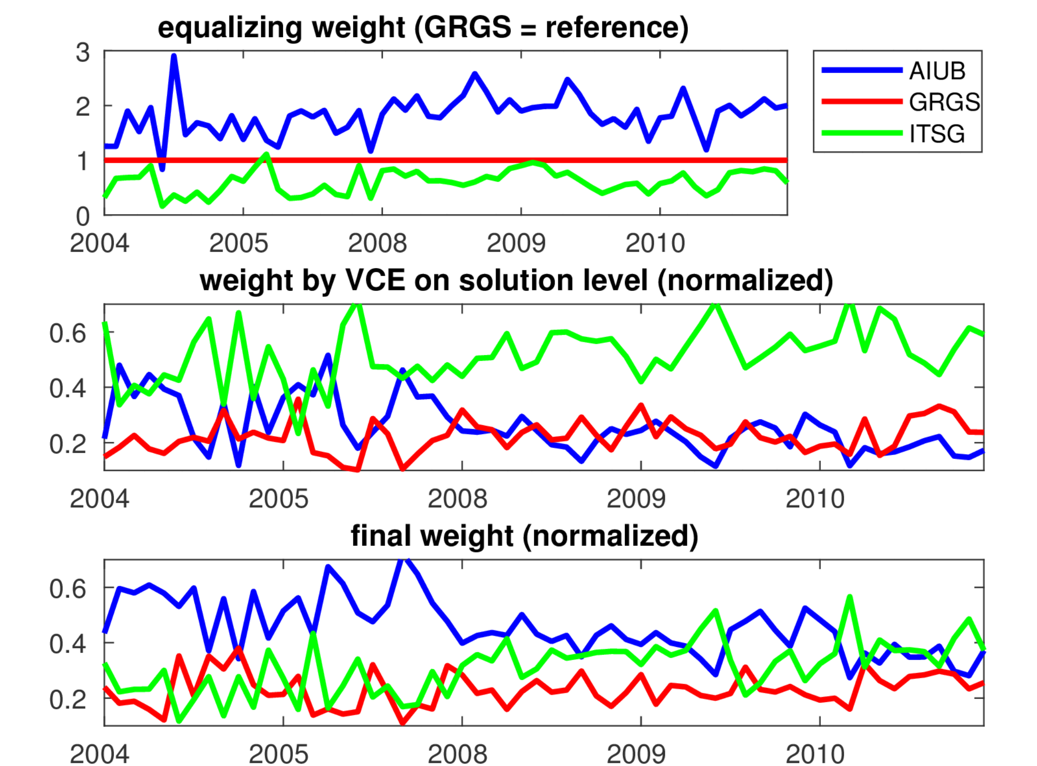
Fig. 7: Relative weights applied for the combination of the NEQs of the extended time-series.
