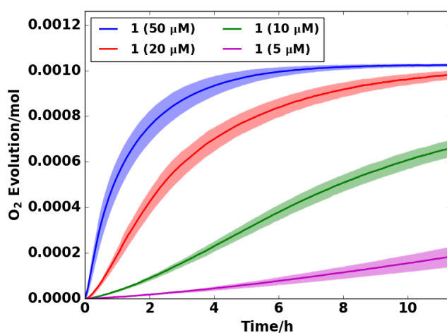
Figure 6. Oxygen evolution traces of the initial 11 h of water oxidation catalyzed by complex 1 at different concentrations (4.5–49.6 \mu\text{M} ; for accurate concentrations of the complex, see Table 1). Solid lines represent the average of multiple measurements. Faded areas illustrate error bands at 95 % confidence interval.
