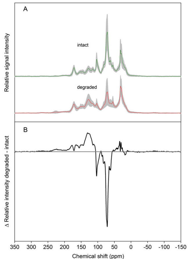
Figure 2. Peat composition revealed by nuclear magnetic resonance spectroscopy. Panel a shows the average ( \pm 1 standard deviation) cross polarization magic angle spinning ^{13}\text{C} nuclear magnetic resonance spectrum for intact and degraded peat. The differential spectrum (panel b) reveals a preferential loss of O-alkyl C (signals at around 72 and 105 ppm) and a selective enrichment of both aliphatic (signal around 30 ppm) and aromatic (130 ppm) C in old peat from drained organic soils relative to intact peats. [Colour figure can be viewed at wileyonlinelibrary.com ]
