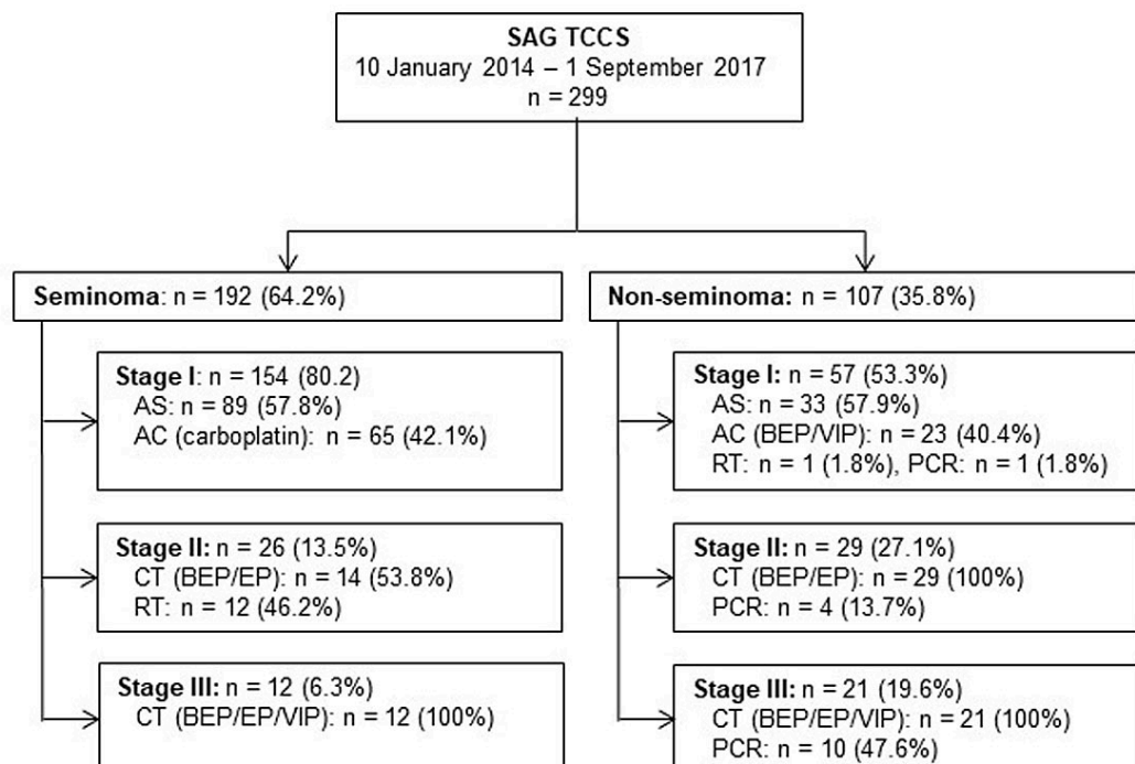
Figure 1: Distribution of GCT patients AC = adjuvant chemotherapy; AS = active surveillance; BEP = bleomycin, etoposide, cisplatin; CT = curative chemotherapy; EP = etoposide, cisplatin; PCR = postchemotherapy resection; RT = radiotherapy; SAG TCCS = Swiss Austrian German Testicular Cancer Cohort Study; VIP = etoposide, ifosfamide, cisplatin.
