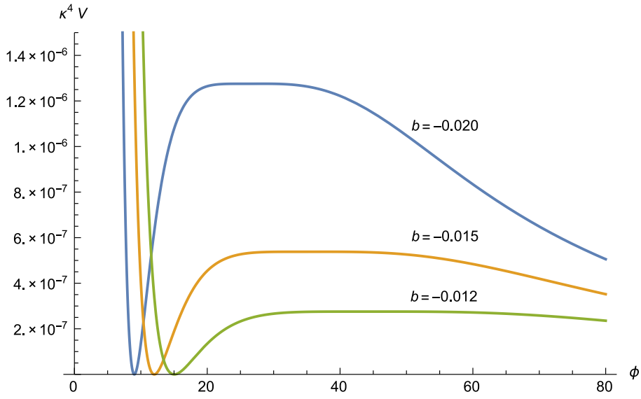
Figure 4: A plot of the scalar potential for p = 2 , with b = -0.020 , b = -0.015 and b = -0.012 . Note that we choose the parameters \alpha and \xi as in eq. (9.4) with c = 0.06 .
