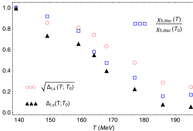
FIG. 2. Comparison between the scaling of \chi_{5,\text{disc}} and the subtracted condensate \Delta_{ls}(T; T_0) in (32), with respect to the reference temperature T_0 = 139 MeV. Data are taken from [4] for 32^3 \times 8 lattice size and \hat{m}/m_s = 0.088 . We include also the comparison with \sqrt{\Delta_{ls}} for the reasons explained in the main text.
