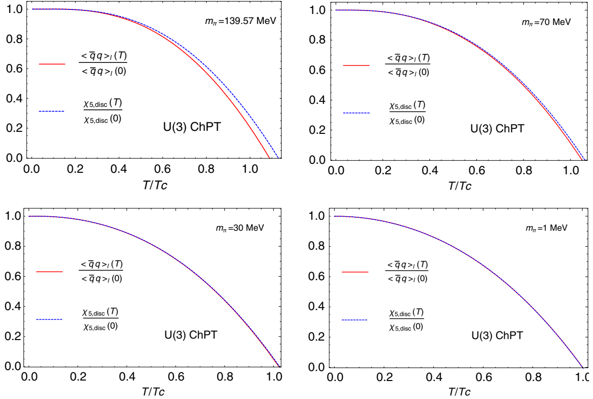
FIG. 9. Comparison of temperature scaling of \chi_{5,\text{disc}} and \langle \bar{q}q \rangle_I(T) for different values of the pion mass.
