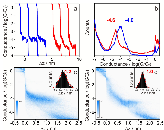
Fig. 1 Single-molecule conductance measurements of 1 and 1-2F . (a) Typical individual conductance - relative distance traces for 1 and 1-2F recorded from conductance measurements at V_{\text{bias}} = 100 mV, blue for 1 and red for 1-2F . (b) One-dimensional (1D) conductance histograms of 1 (blue) and 1-2F (red). (c,d) Two-dimensional (2D) conductance histograms and stretching distance \Delta z distributions (inset) of 1 (c) and 1-2F (d).
