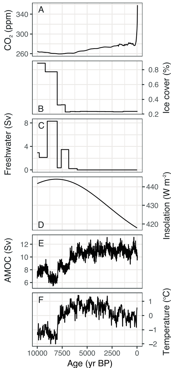
Figure 4. Climate forcings and simulated Arctic temperature and AMOC variability over the past 10 kyr. (a) CO 2 concentration. (b) Fraction of Northern Hemisphere land covered by ice. (c) Northern Hemisphere freshwater forcing. (d) June–August mean insolation at 65°N. (e) Atlantic Meridional Overturning Circulation (maximum MOC in the North Atlantic). And (f) area-weighted mean annual temperature anomaly north of 60°N. Data sources are given in the description of the model setup in section 2. AMOC = Atlantic Meridional Overturning Circulation.
