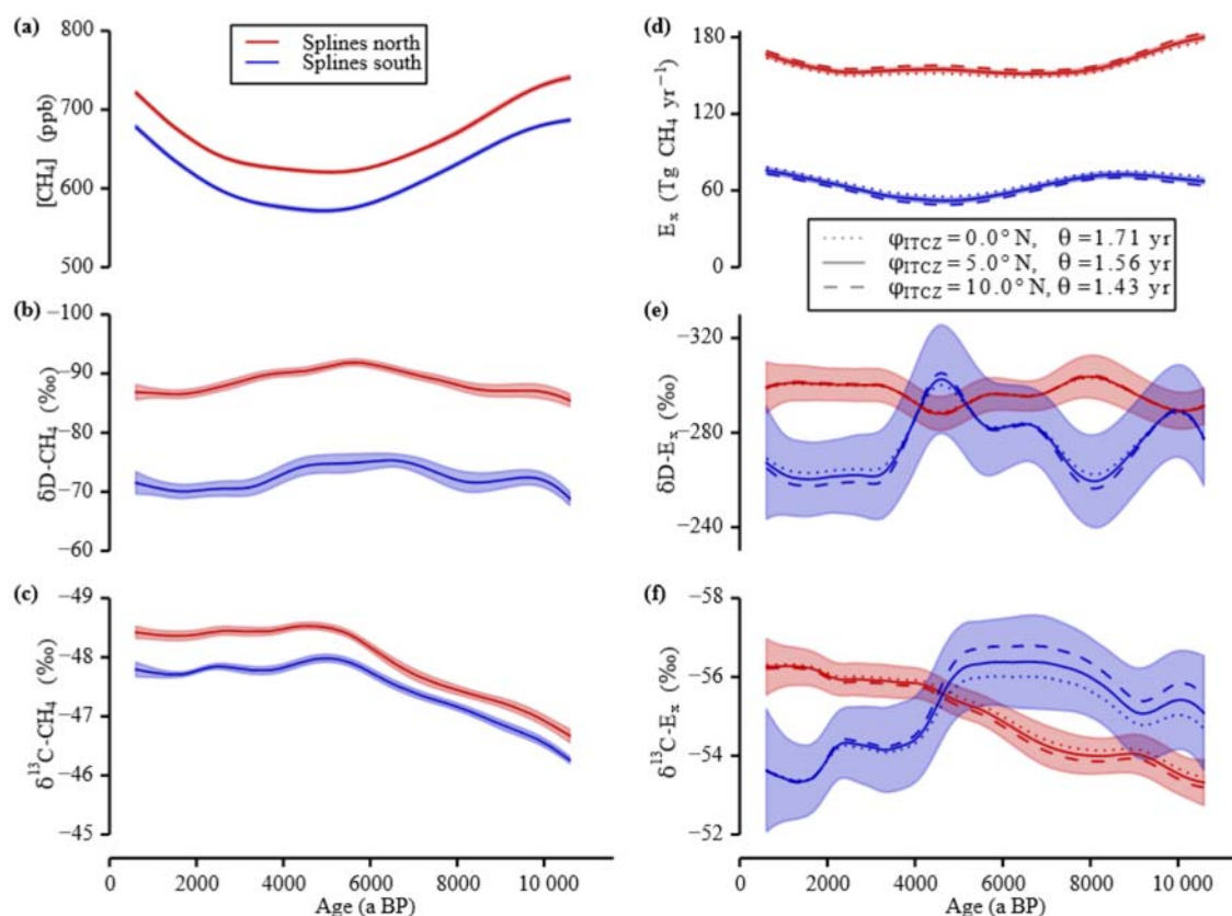
Figure 5. Sensitivity study “SF 6 calibration”. In panels (a–c) the data splines with the 1 \sigma uncertainty bands of the measured tropospheric values are shown. In panels (d–f) the calculated strengths and the isotopic signature of the emissions are shown for the three different \phi_{ITCZ} and \theta set-ups to investigate the sensitivity of the inversion to the SF 6 calibration. Note the inverted y axes in panels (b), (c), (e), and (f).
