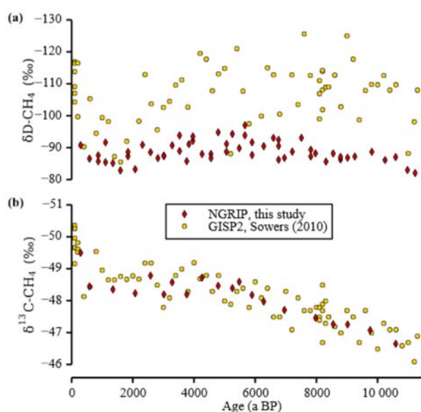
Figure 4. Comparison of stable \text{CH}_4 isotope data. This study's stable \text{CH}_4 isotope values of the NGRIP ice cores are shown together with the data published by Sowers (2010) using the GISP2 ice core. The \delta\text{D-CH}_4 data sets (a) differ in the absolute level and the variance, whereas the \delta^{13}\text{C-CH}_4 data (b) are in good agreement. Note that all data are corrected for gravitational fractionation in the firn column. All data of this study are free of krypton interference, whereas the GISP2 \delta^{13}\text{C-CH}_4 record has been subsequently corrected for it (Schmitt et al., 2013). Note the inverted y axes.
