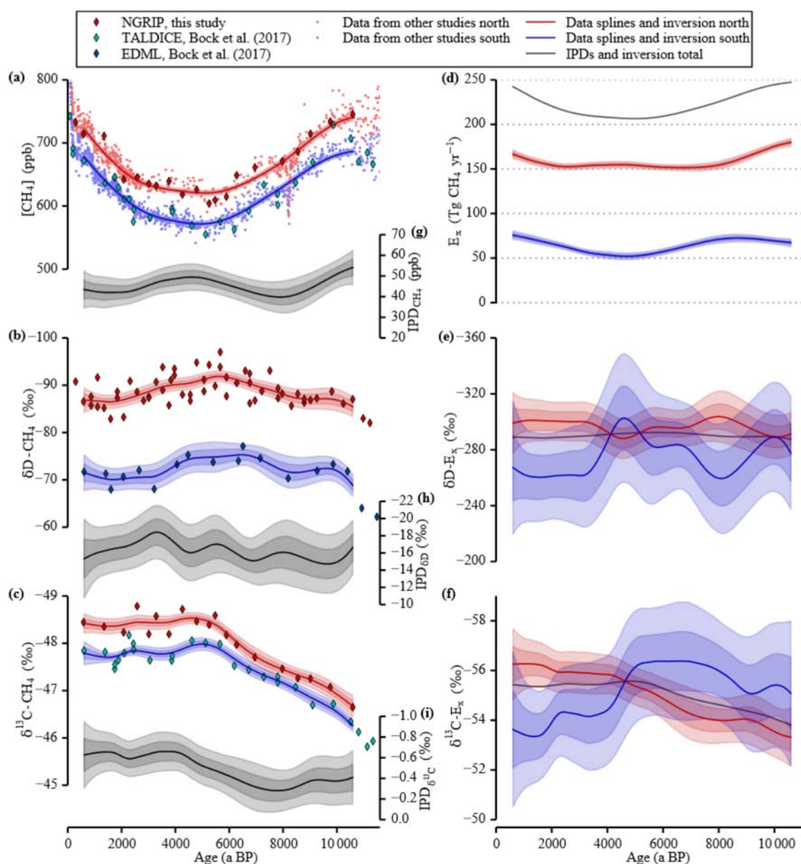
Figure 3. Data and inversion. The panels on the left (a–c) show the concentration and the two stable isotope signatures of \text{CH}_4 measured in ice cores representing the tropospheric values over the Holocene. The concentration data are complemented with data from other studies (see Table 1). All three parameters were measured on ice cores from Greenland (red) and from Antarctica (blue and cyan) representing the northern and the southern polar troposphere, respectively. A spline function with a cut-off period of 3000 years has been used to calculate the smoothed evolution of the tropospheric signals represented by the lines and the 1\sigma and 2\sigma error bands. The panels (g), (h), and (i) show the IPDs of all three parameters also with their 1\sigma and 2\sigma error bands. A box model inversion is used to calculate the hemispheric \text{CH}_4 emissions shown in the panels on the right. In panel (d) the emission strengths are shown for both hemisphere boxes together with the total \text{CH}_4 emissions. Panels (e) and (f) show the mean isotopic signatures of the emissions for both stable isotopes of \text{CH}_4 . All the error bands represent 1\sigma and 2\sigma uncertainties. Note the inverted y axes in panels (b), (c), (e), (f), (h), and (i). Red refers to Northern Hemisphere records and blue to Southern Hemisphere records throughout the paper.
