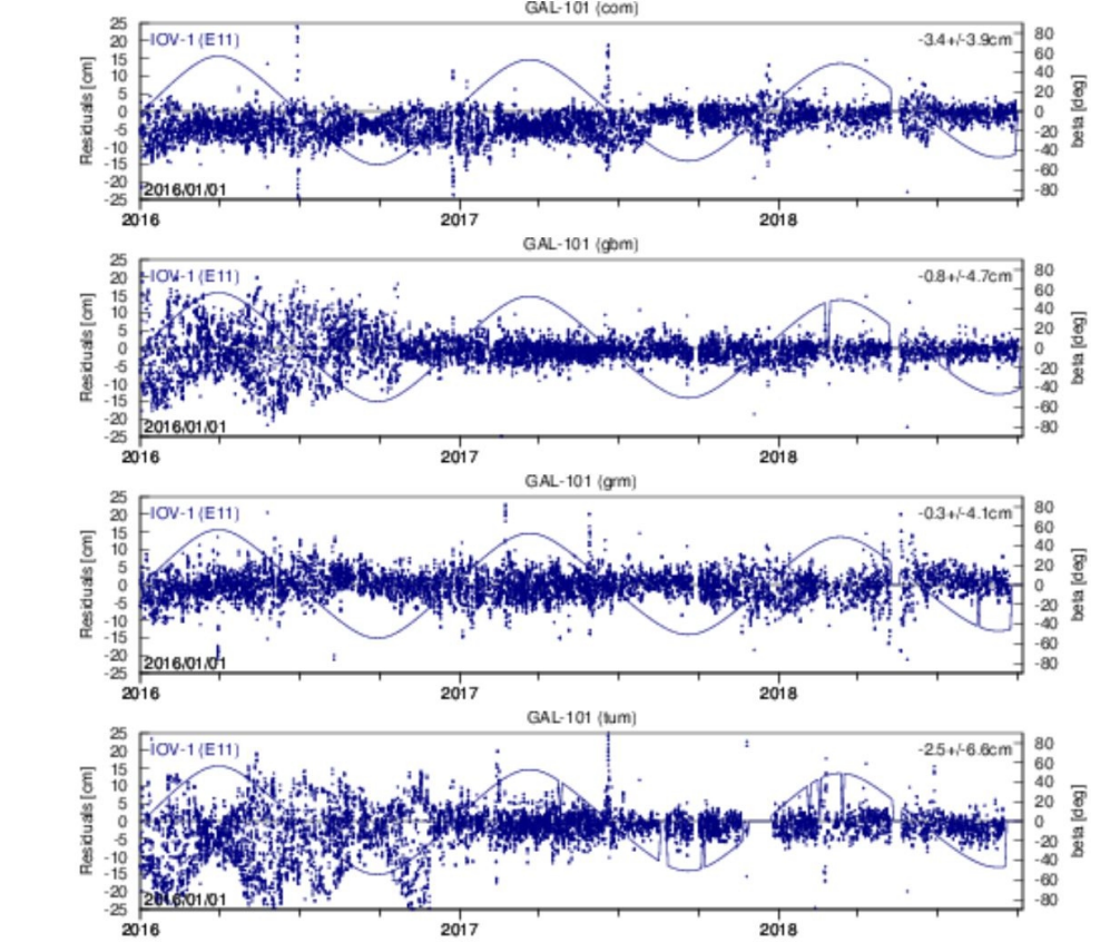
Fig. 4: SLR assessment of E11 orbits computed by four analysis centers (URL: http://mgex.igs.org ). The scatter of SLR residuals is elevated during eclipse seasons.
