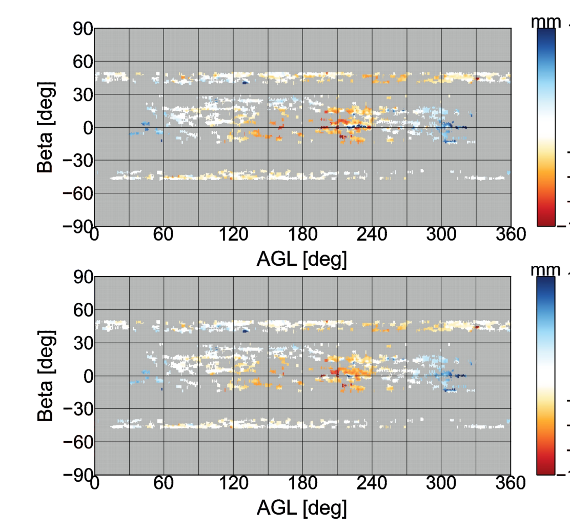
Fig. 11: SLR residuals of Galileo orbits computed using ECOM2 (top) and adjusted ECOM2 (bottom) over days 70-101 of 2018.
