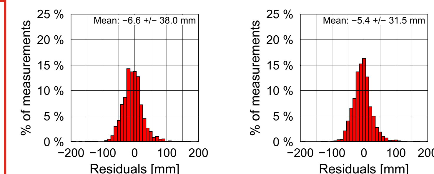
Fig. 12: Histograms of SLR residuals of Galileo orbits computed using ECOM2 (left) and adjusted ECOM2 (right) over days 70-101 of 2018.
