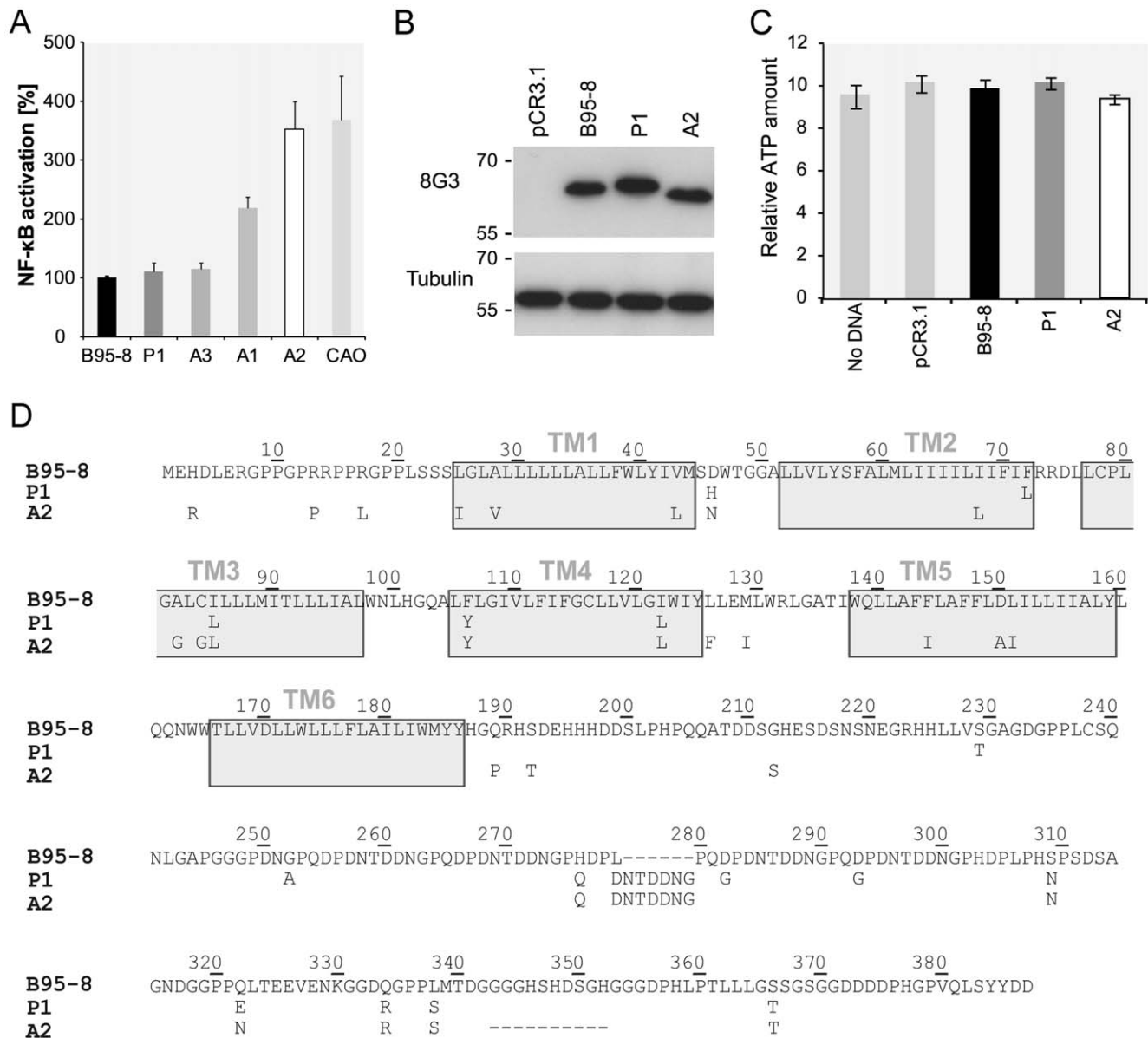
Figure 1. Analysis of LMP1 variants. (A) NF-κB activation by LMP1 variants. 293T cells were transfected with 50 ng of expression vector coding for LMP1 prototype (B95-8) and variants (P1, A3, A1, A2, CAO) and 50 ng of Firefly luciferase reporter plasmid. An analogous strategy of subcloning was applied to variants, prototype and CAO LMP1, to ensure appropriate comparisons. NF-κB activity was measured twenty hours after transfection using luciferase assay (Promega). Data are mean \pm SD of triplicates and shown is a representative of three independent experiments with similar results. (B) Expression of LMP1 B95-8, A2 and P1 was visualized by SDS-PAGE and Western blotting with anti-LMP1 8G3 antibody. Detection against tubulin was used as internal control. (C) Measure of the toxicity of LMP1 variants. Cells were transfected with 50 ng of LMP1 B95-8, P1 or A2. Untransfected cells and cells transfected with empty vector were used as experimental controls. ATP amount was measured 24 hours after transfection using CellTiter-Glo Luminescent Cell Viability Assay (Promega). Shown is a representative experiment of three independent experiments with similar results. (D) Amino acid sequence alignment of B95-8, P1 and A2 LMP1. Only amino acids that differ from the sequence of prototype B95-8 LMP1 are indicated. Transmembrane segments are indicated by light gray boxes and deletions by dashes. doi:10.1371/journal.pone.0032168.g001
