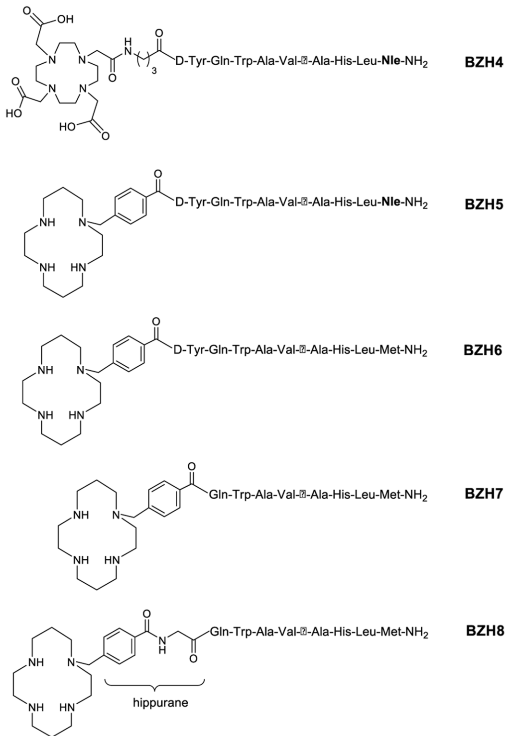
Figure 2. Scheme of modification on BN peptide to optimize affinity unit, form hippurane-like spacer and to functionalize for radiolabeling with 64/67 Cu and 111 In.
