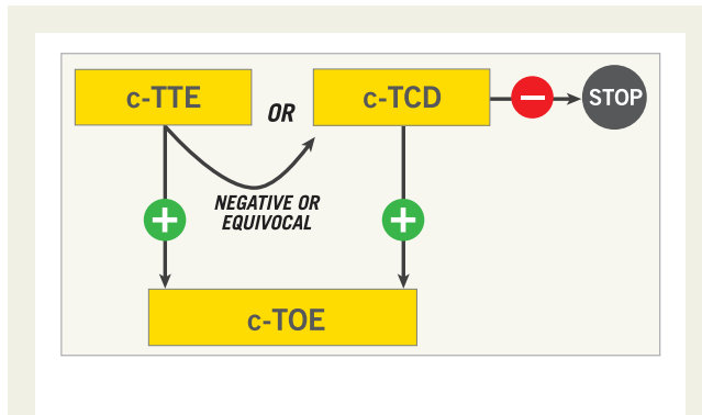
Figure 1 Algorithm for the diagnosis of PFO. c-TCD: contrast-enhanced transcranial Doppler; c-TOE: contrast-enhanced transoesophageal echocardiography; c-TTE: contrast-enhanced transthoracic echocardiography; –negative test for the presence of right-to-left shunt; +positive test for the presence of right-to-left shunt.
