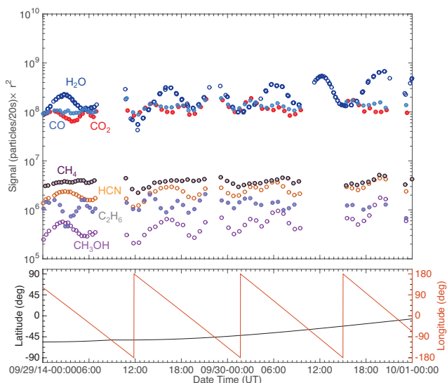
Fig. 1: Top: Typical pre-inbound-equinox (29-30 September 2014) southern hemisphere time variation of the seven studied species for a time period analyzed in ALK15. The signal has been scaled to the distance of Rosetta from the center of the nucleus (i.e., multiplied by r^2 ). Species that trend together are illustrated with empty and filled markers. Bottom: Corresponding sub-spacecraft longitude (red) and latitude (black). Errors are smaller than the marker size. Plot shown for comparative purposes with post-outbound-equinox data.
