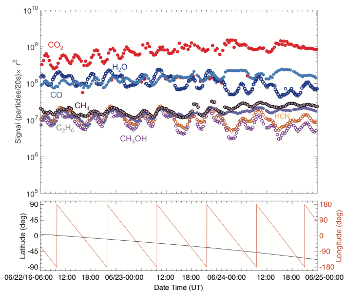
Fig. 2: Top: Post-outbound-equinox (22-24 June 2016) southern hemisphere time variation of the seven studied species scaled to the distance of Rosetta from the center of the nucleus ( r^2 ), and the corresponding sub-spacecraft longitude and latitude values (bottom). Species that trend together are illustrated with empty and filled markers. Errors are smaller than the marker size.
