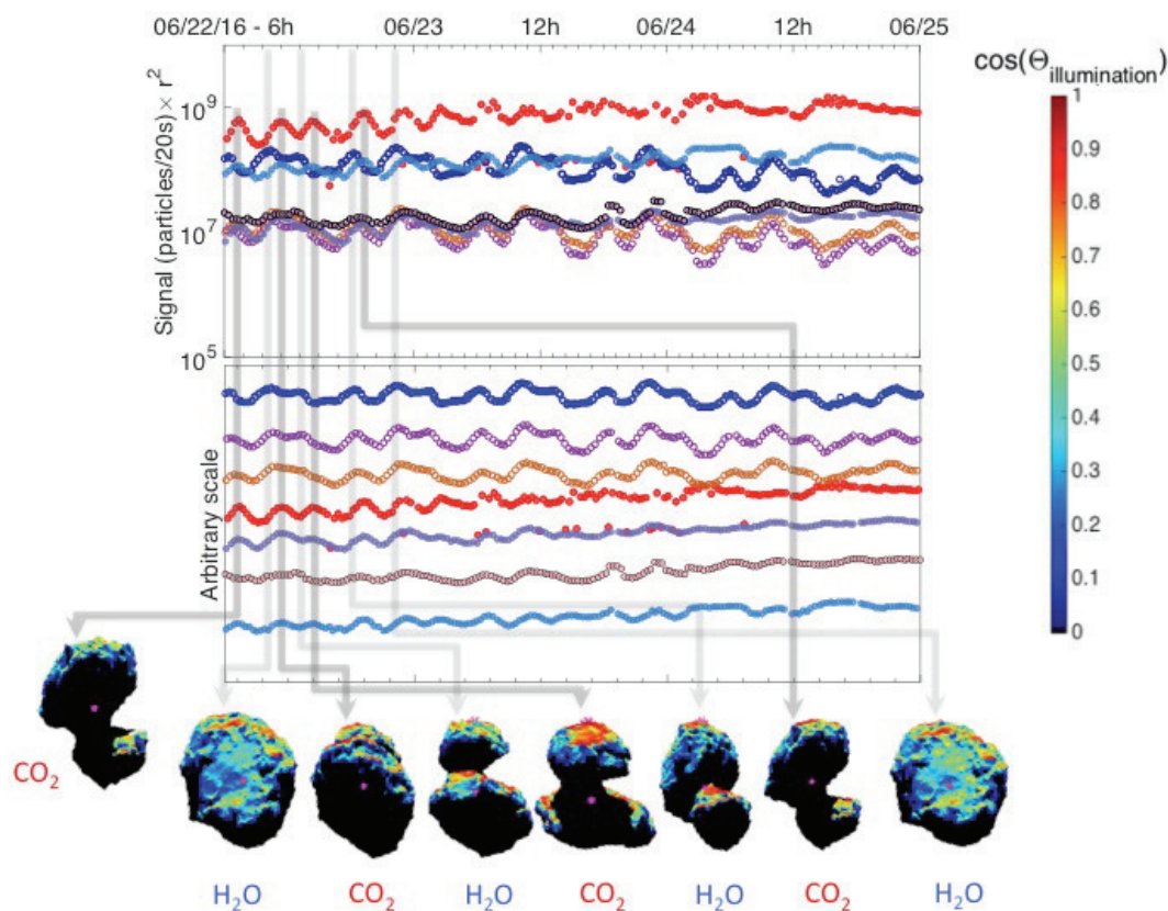
Fig. 10: Snapshots of the post-equinox spacecraft view of 67P at the times of signal maxima with the rough illumination (the cosine between the surface normal and the direction of the Sun). Top: Signal corrected for r^2 . Bottom: Shifted signal according to volatility. Light gray arrows indicate \text{H}_2\text{O} , while darker gray arrows indicate \text{CO}_2 maxima. Shape model: ESA NAVCAM.
