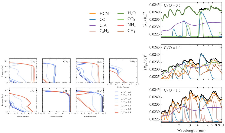
Fig. 13 Left: Vertical abundance profiles for different molecules for a range of C/O. The different coloured lines show the molar fraction profiles at different C/O, as shown by the legend. Right: synthetic transit spectra and contribution of the various opacities for the atmospheric compositions shown on the left (Rocchetto et al. [193])
