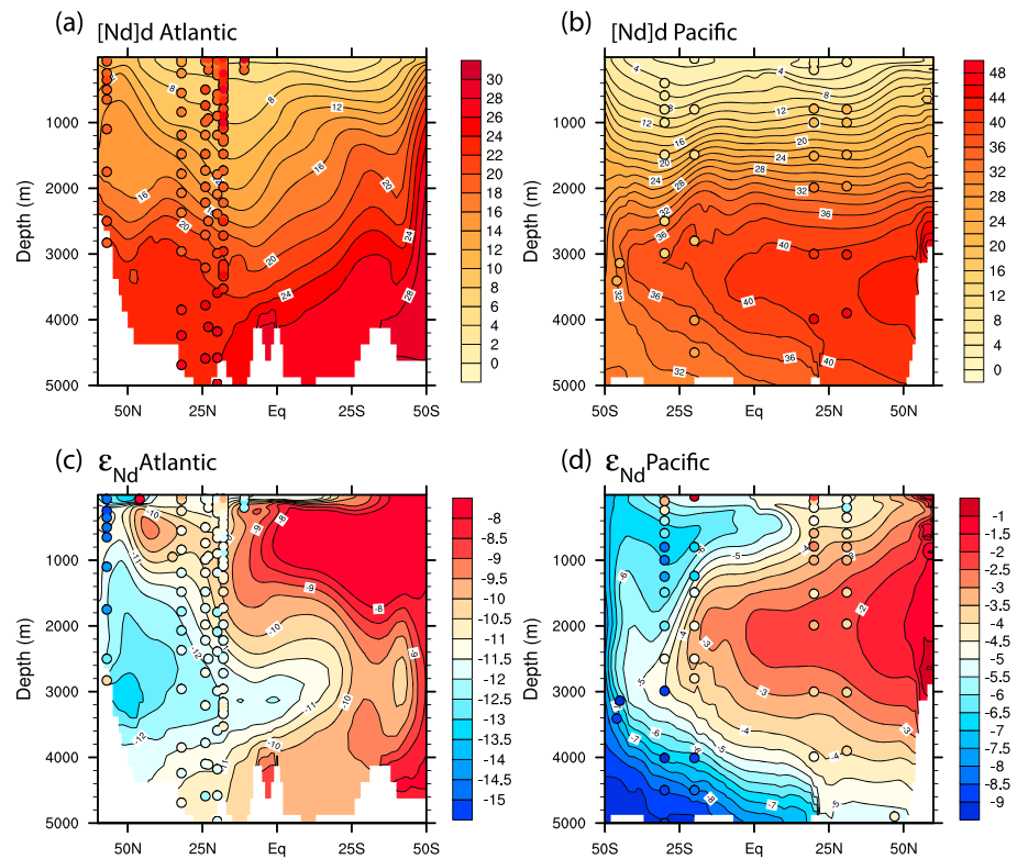
Figure 1. Nd concentration (a and b) and \epsilon_{\text{Nd}} (c and d) in the vertical section in the Atlantic (20–30°W) and the Pacific (150–160°W) in CTRL. Observations (from the same regions) are superimposed as filled circles using the same color scale.
