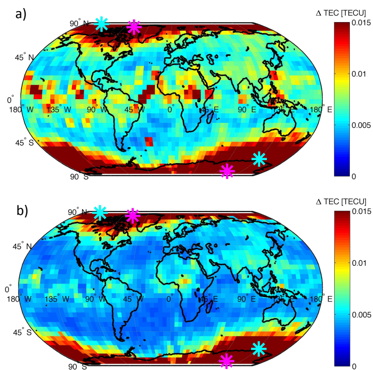
Figure 3. a) Global map of f \Delta\text{TEC} during September 2013 obtained by the arithmetic mean of the values in the binned cells. b) Global map of \Delta\text{TEC} during September 2013 obtained by the median of the values in the binned cells. The geomagnetic (magnetic) poles are indicated by the magenta (cyan) star symbols respectively.
