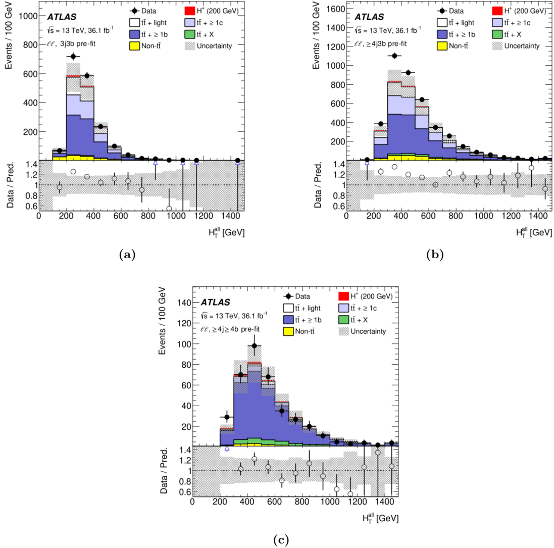
Figure 4. Distributions of the H_T^{\text{all}} variable before the fit to the data in the three SRs of the \ell\ell channel: (a) 3j3b , (b) \geq 4j3b and (c) \geq 4j\geq 4b . Each background process is normalised according to its cross-section and the normalisation of the t\bar{t} + \geq 1b and t\bar{t} + \geq 1c backgrounds corresponds to the prediction from POWHEG+PYTHIA8 for the fraction of each of these components relative to the total t\bar{t} prediction. The t\bar{t} + X includes contributions from t\bar{t}W , t\bar{t}Z and t\bar{t}H . In addition, the expectation for a 200 GeV signal is shown for a cross-section times branching ratio of 1 pb. The lower panels display the ratio of the data to the total prediction. The hatched bands show the pre-fit uncertainties. The level of agreement is improved post-fit due to the adjustment of the normalisation of the t\bar{t} + \geq 1b and t\bar{t} + \geq 1c backgrounds and the other nuisance parameters by the fit.
