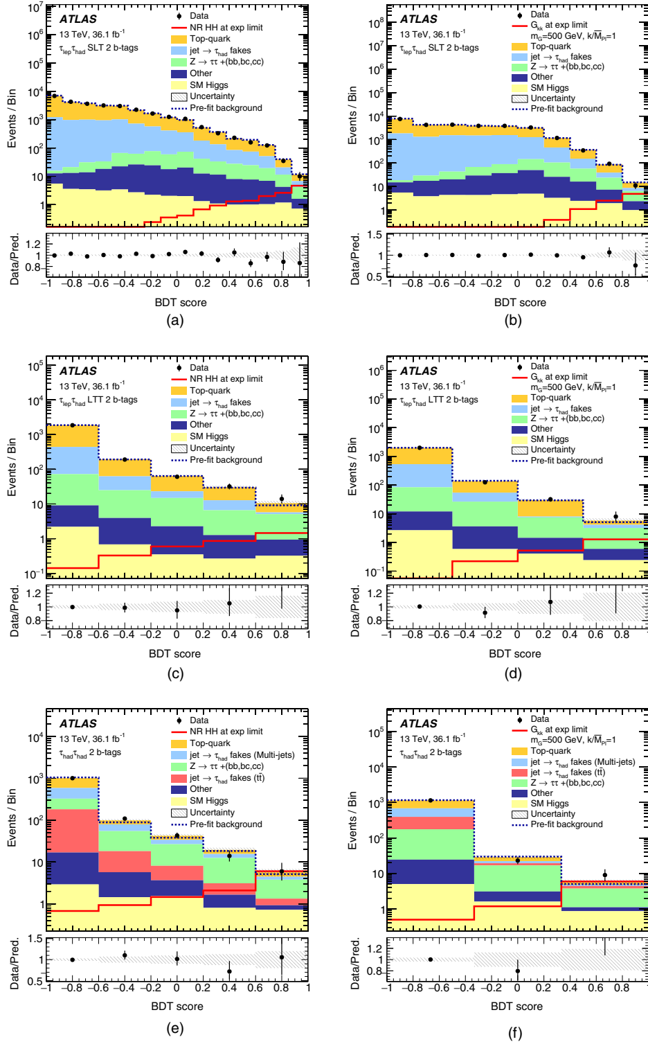
FIG. 1. Distributions of the BDT score for NR HH signal (left) and bulk RS signal with m_{G_{KK}} = 500 GeV and k/\bar{M}_{\text{Pl}} = 1 (right) in the (a),(b) \tau_{\text{lep}}\tau_{\text{had}} single-lepton trigger (SLT), (c),(d) lepton + \tau_{\text{had}} trigger (LTT) and (e),(f) \tau_{\text{had}}\tau_{\text{had}} channels. Distributions are shown after the fit to the background-only hypothesis and the signal is scaled to approximately the expected limit. The hatched band indicates the combined statistical and systematic uncertainty in the background. The ratio of the data to the sum of the backgrounds is shown in the lower panel.
