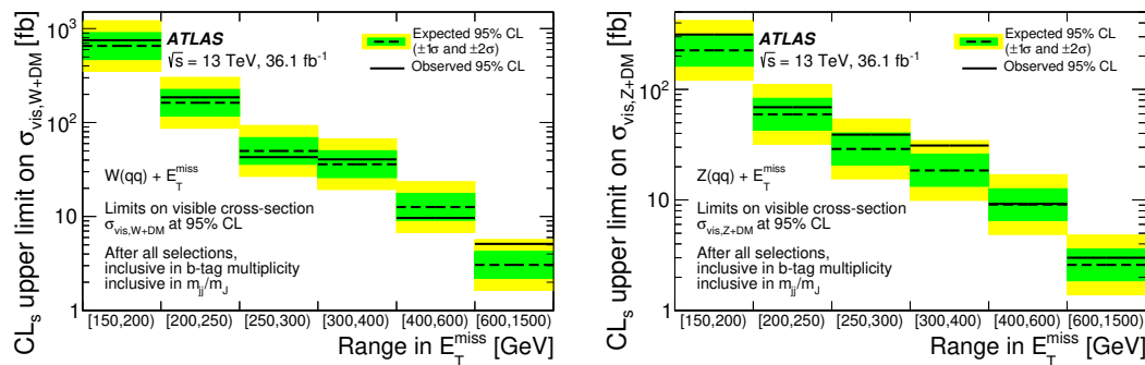
Figure 10. Upper limits at 95% CL on the visible cross section \sigma_{\text{vis}, W+DM} (left) and \sigma_{\text{vis}, Z+DM} (right) in the six E_T^{\text{miss}} regions, after all selection requirements, but inclusive in the b -tag multiplicity and the W/Z candidate mass m_{jj}/m_J . The observed limits (solid line) are consistent with the expectations under the SM-only hypothesis (dashed line) within uncertainties (filled bands).
