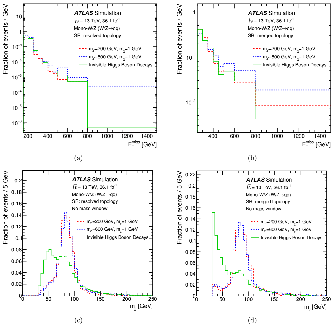
Figure 2. Expected distributions of missing transverse momentum, E_T^{\text{miss}} , normalized to unit area, for the simplified vector-mediator model and invisible Higgs boson decays after the full selection in the (a) resolved and (b) merged event topologies, and the expected invariant mass distributions (c) m_{jj} in the resolved and (d) m_J in the merged event topologies, before the mass window requirement. The signal contributions from each resolved (merged) category are summed together. The invisible Higgs boson decays include a large contribution from ggH events, which results in the observed mass distribution.
