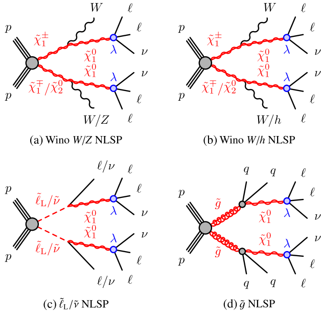
FIG. 1. Diagrams of the benchmark SUSY models of RPC NLSP pair production of (a) and (b) a wino, (c) slepton/sneutrino and (d) gluino, followed by the RPV decay of the \tilde{\chi}_1^0 LSP. The LSP is assumed to decay as \tilde{\chi}_1^0 \rightarrow \ell\ell\nu with 100% branching ratio.
