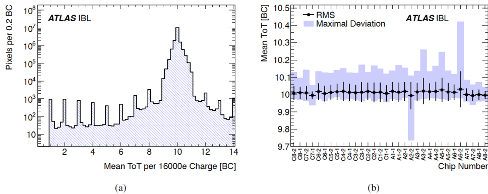
Figure 37. (a) One-dimensional Time-over-Threshold (ToT) distribution for all pixels when tuned to 10 ToT, using an injected charge of 16\,000\,e^- . The spikes result from injection failures where the selected ToT value is not 10. Non-integer mean ToT values result when successive injections to evaluate the mean select differing ToT values. (b) The average ToT distribution as a function of the chip number (position) on the stave. The data are from all 18 qualified staves using a mean module threshold of 1500\,e^- at -12^\circ\text{C} .
