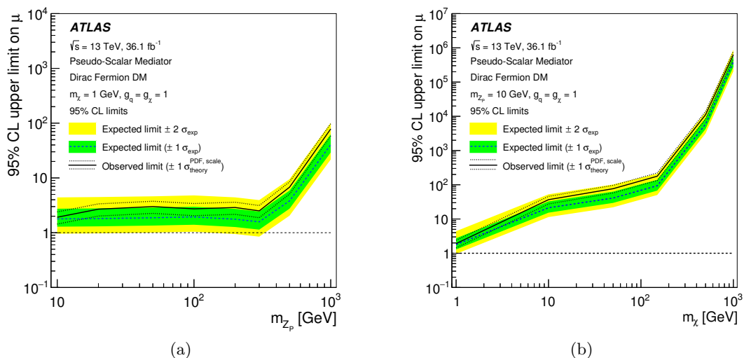
Figure 7. Observed and expected 95 % CL limits on the signal strength \mu \equiv \sigma^{95\% \text{ CL}}/\sigma as a function of (a) the mediator mass for a very light WIMP and (b) the WIMP mass for m_{Z_P} = 10 \text{ GeV} , in a model with spin-0 pseudoscalar mediator and g_q = g_\chi = 1.0 . The bands indicate the \pm 1\sigma theory uncertainties in the observed limit and the \pm 1\sigma and \pm 2\sigma ranges of the expected limit in the absence of a signal.
