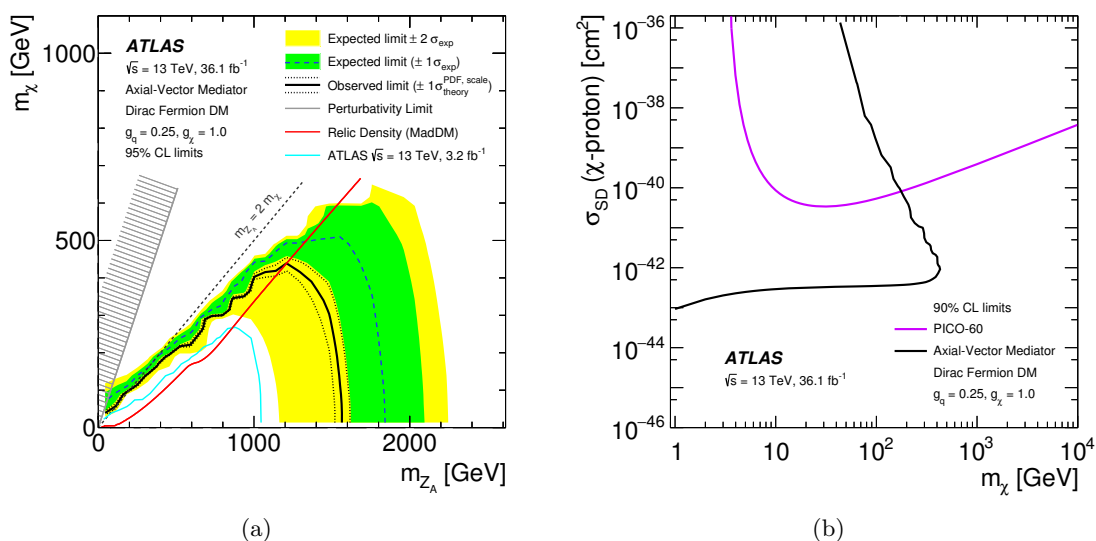
Figure 5. (a) Axial-vector 95% CL exclusion contours in the m_{Z_A} - m_{\chi} parameter plane. The solid (dashed) curve shows the observed (expected) limit, while the bands indicate the \pm 1\sigma theory uncertainties in the observed limit and \pm 1\sigma and \pm 2\sigma ranges of the expected limit in the absence of a signal. The red curve corresponds to the set of points for which the expected relic density is consistent with the WMAP measurements (i.e. \Omega h^2 = 0.12 ), as computed with MADDM [94]. The region on the right of the curve corresponds to higher predicted relic abundance than these measurements. The region excluded due to perturbativity, defined by m_{\chi} > \sqrt{\pi/2} m_{Z_A} , is indicated by the hatched area. The dotted line indicates the kinematic limit for on-shell production m_{Z_A} = 2 \times m_{\chi} . The cyan line indicates previous results at 13 TeV [1] using 3.2 \text{ fb}^{-1} . (b) A comparison of the inferred limits (black line) to the constraints from direct detection experiments (purple line) on the spin-dependent WIMP-proton scattering cross section in the context of the simplified model with axial-vector couplings. Unlike in the m_{Z_A} - m_{\chi} parameter plane, the limits are shown at 90% CL. The results from this analysis, excluding the region to the left of the contour, are compared with limits from the PICO [95] experiment. The comparison is model-dependent and solely valid in the context of this model, assuming minimal mediator width and the coupling values g_q = 1/4 and g_{\chi} = 1 .
