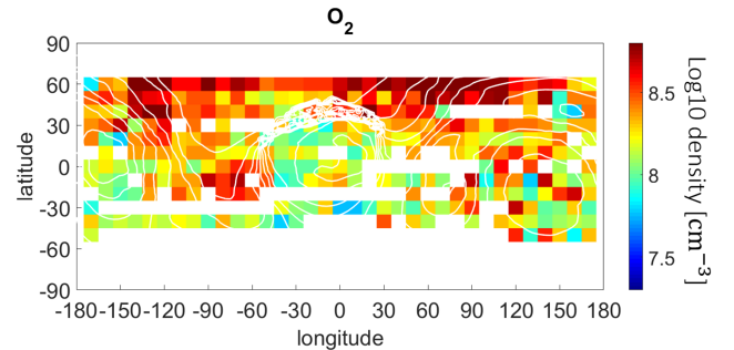
Fig. 8: Spatial heterogeneities of O 2 density (scaled to a distance of 1 km) in cm -3 .km 2 during period A.
