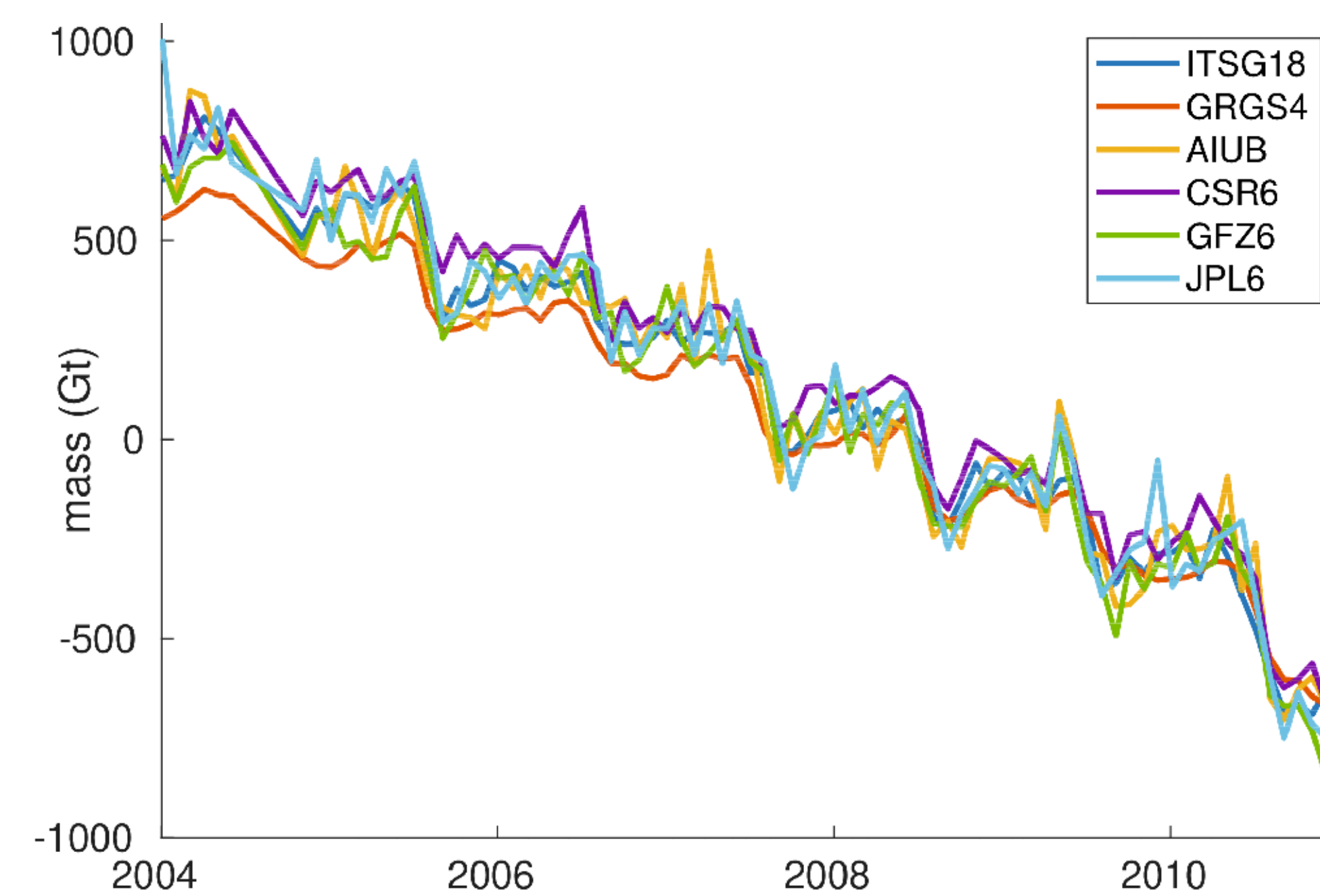
Figure 3: Mass change over Greenland. Only degrees 3 to 90 were taken into account and no Gaussian filter or corrections for leakage and GIA were applied. The attenuated trend visible in the GRGS-RL04 time-series may be related to the regularization by truncation of the eigenvalues in the inversion step.
