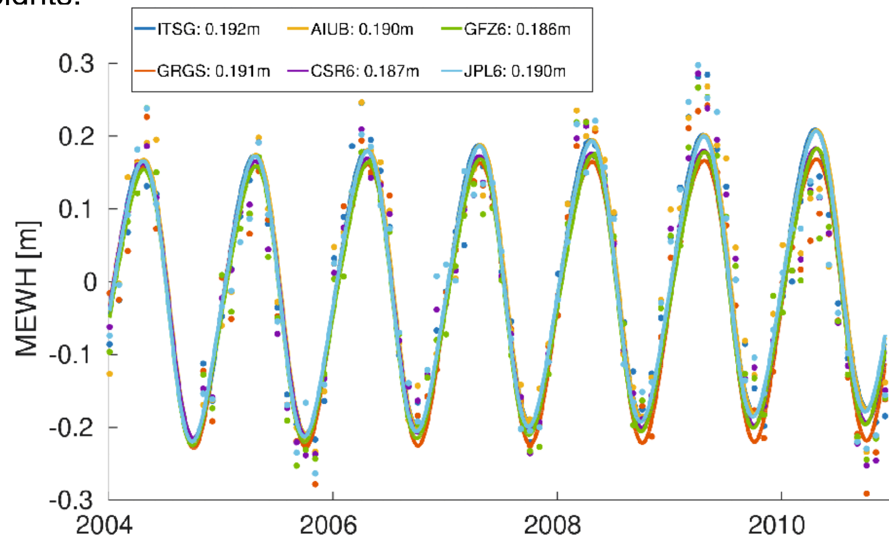
Figure 1: Mean equivalent water heights (MEWH) over the Amazon basin derived from the individual monthly solutions (dots) and from a posteriori fitting trends and seasonal signals (lines). Annual amplitudes, as given in the legend, agree well with each other.
